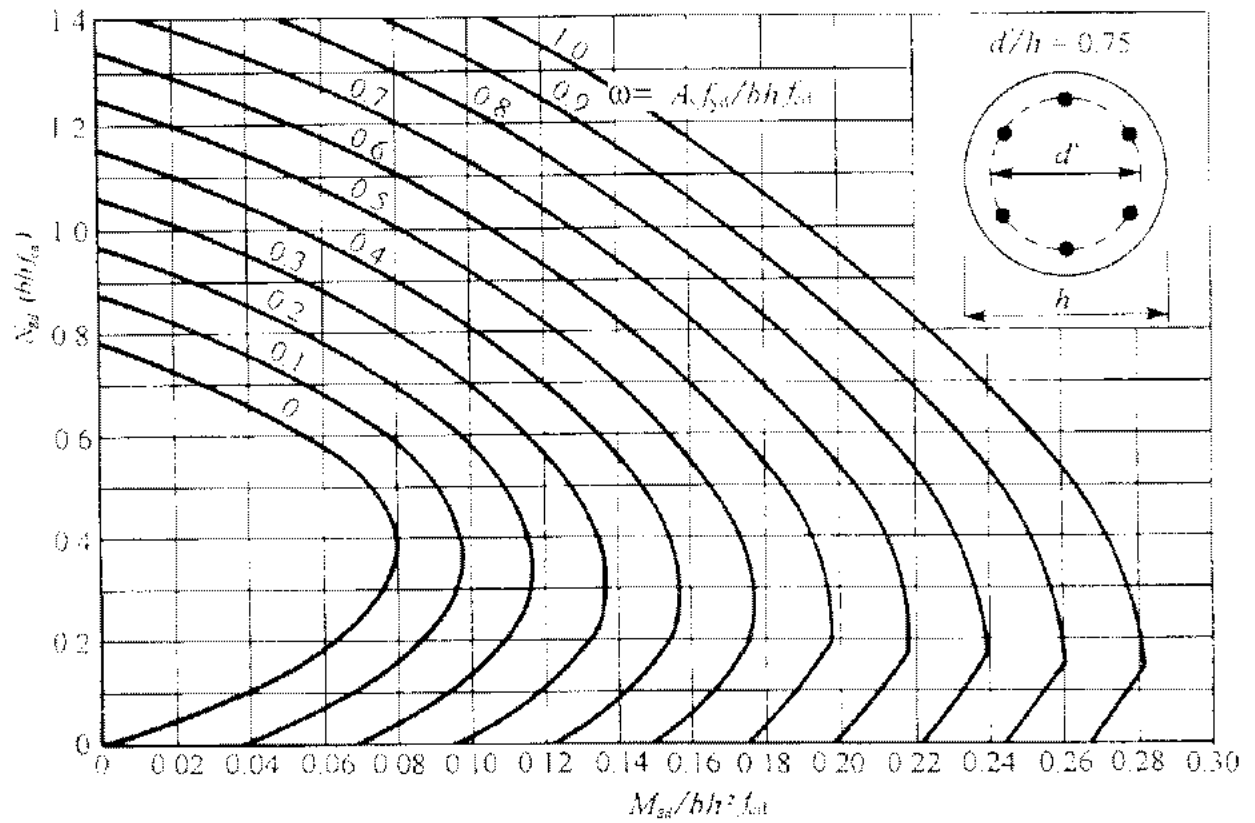
Nomogram 12.7
