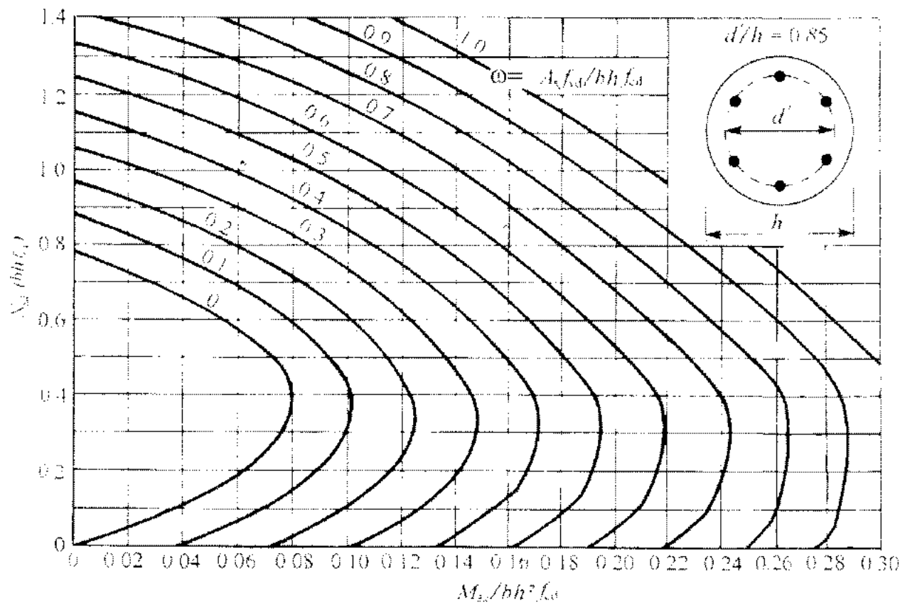
Nomogram 12.9
