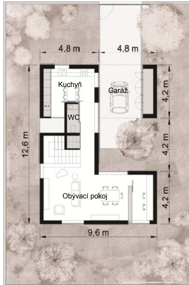
Ground-floor level
