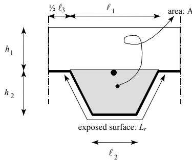
Fig. D.1 : Definition of the rib geometry factor A/L_r for ribs of composite slabs.
