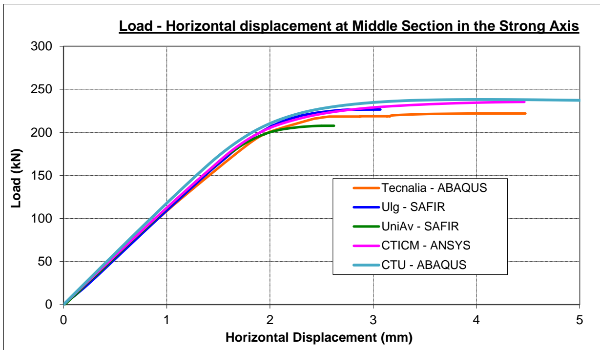
Figure 26: Load – horizontal displacement at middle section in the strong axis for 4 th example
