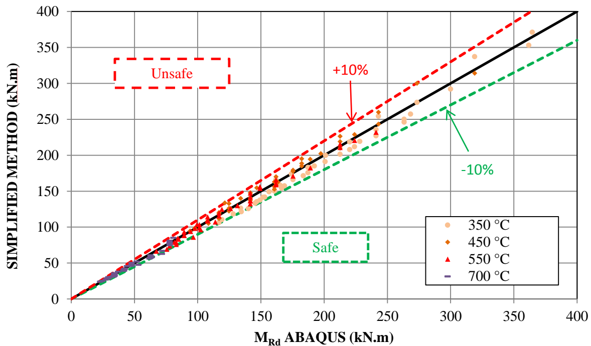
Figure 52: Comparison between numerical analysis and modified new simple design rule for bending moment resistance for steel grade S460
