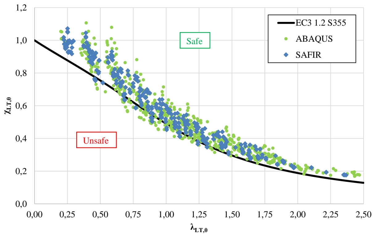
Figure 73: Comparison between FEM LTB curve and LTB curve from EN 1993-1-2 for S355 steel grade
