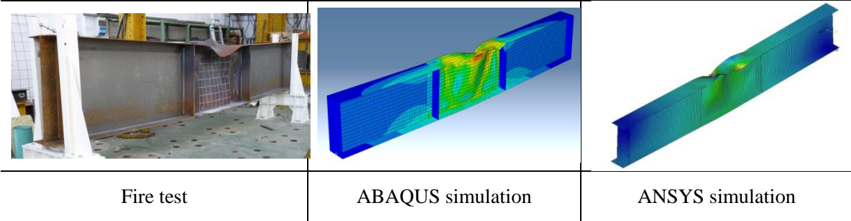
Figure 2: Failure mode shape of the fourth test of simple bending – 650 °C
