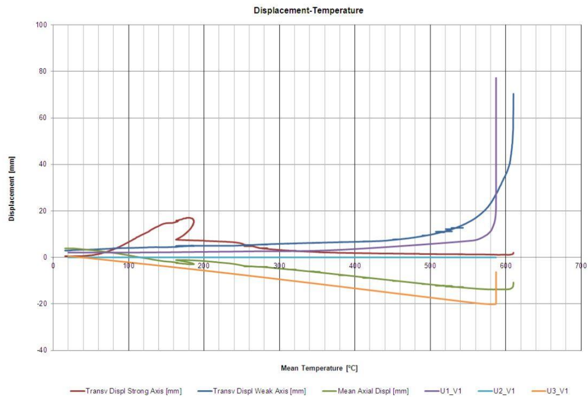
Figure 106: Displacements (mm) in function of temperature (°C) – ABAQUS comparison
