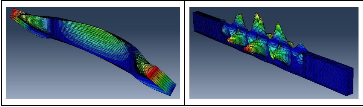
Figure 63: Mode shape from linear buckling analysis: left) lateral torsional buckling failure mode, right) local buckling failure mode
