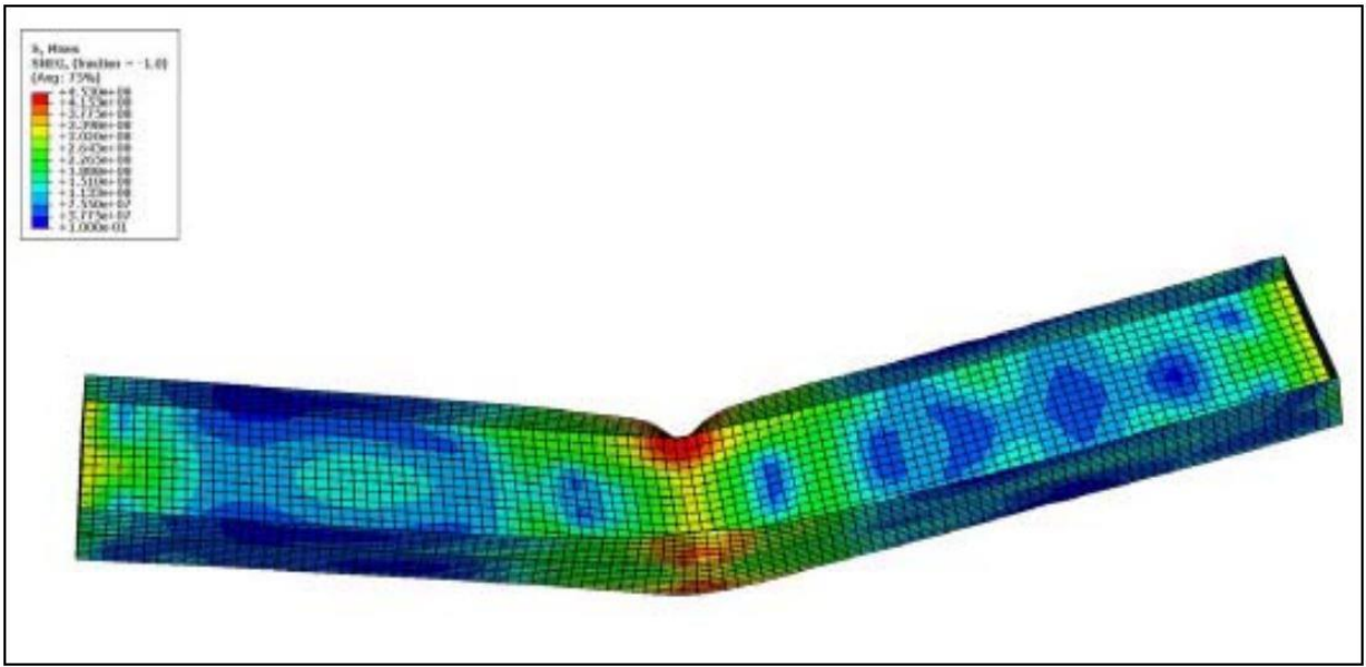
Figure 116: Numerical failure mode obtained with ABAQUS
