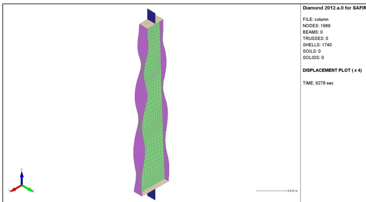
Figure 119: Numerical failure mode obtained with SAFIR
