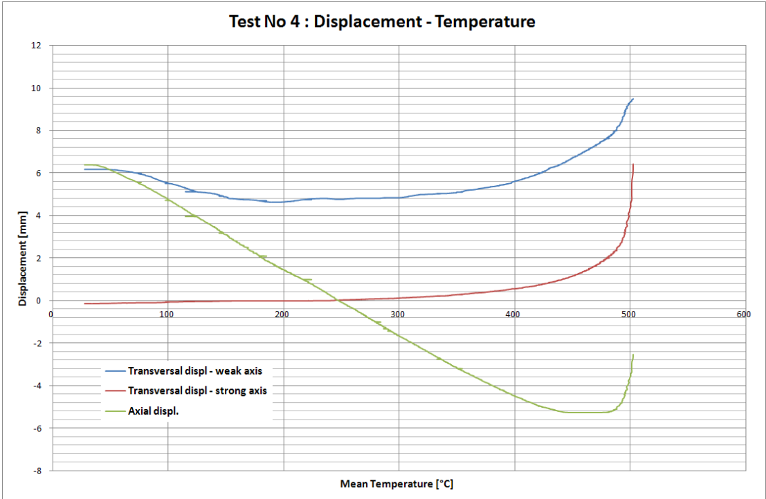
Figure 103: Displacements (mm) in function of the mean temperature (°C)
