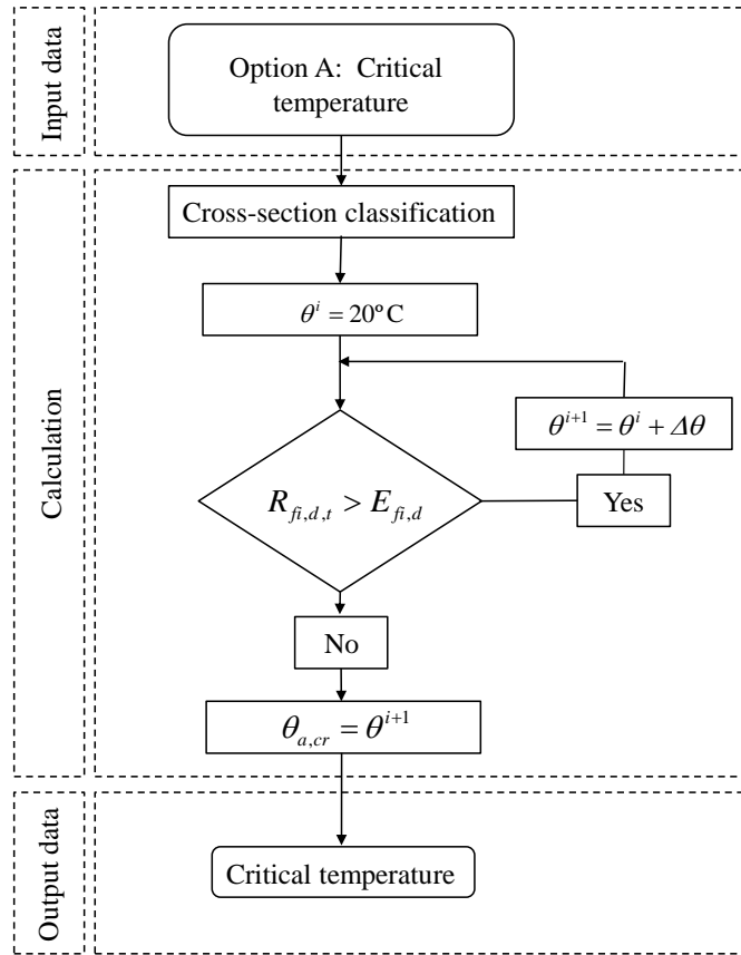
Figure 140: Option A: Calculation flowchart for evaluating the critical temperature
