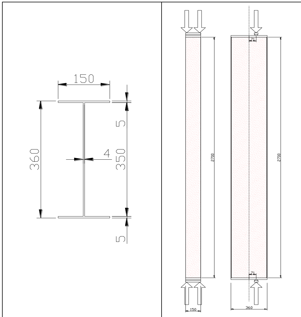
Figure 125: Cross-section design and global design of the tests 5
