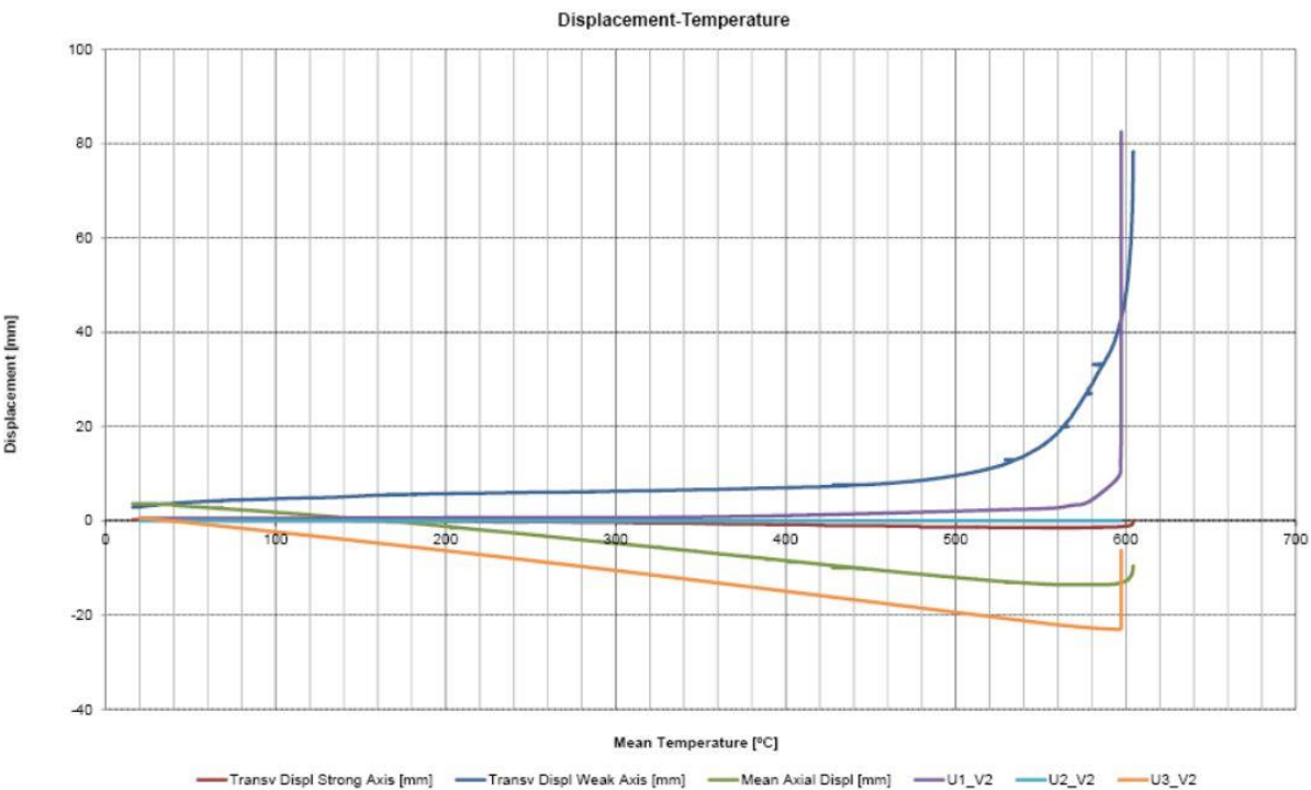
Figure 110: Displacements (mm) in function of temperature (°C) – ABAQUS comparison
