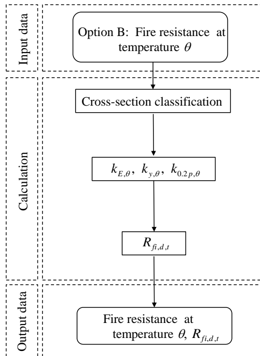
Figure 141: Option B: Calculation flowchart for checking the fire resistance
