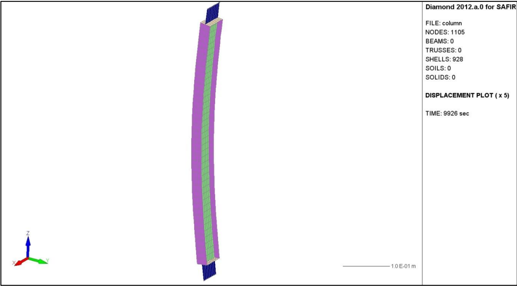
Figure 107: Numerical failure mode obtained with SAFIR
