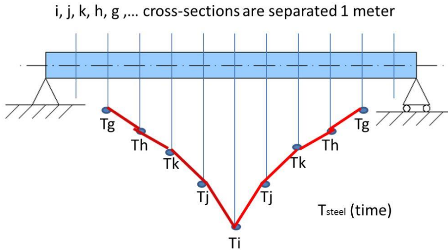
Figure 147: Temperature distribution in different sections of a beam
