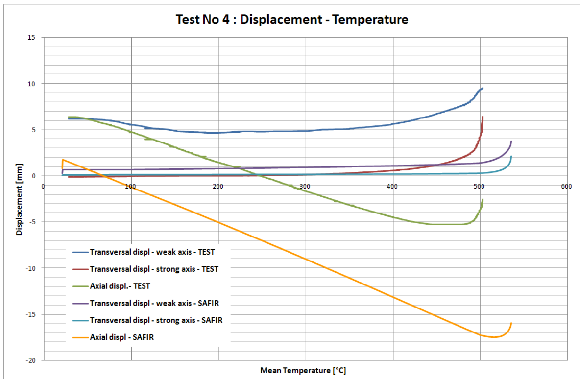
Figure 117: Displacements (mm) in function of temperature (°C) – SAFIR comparison
