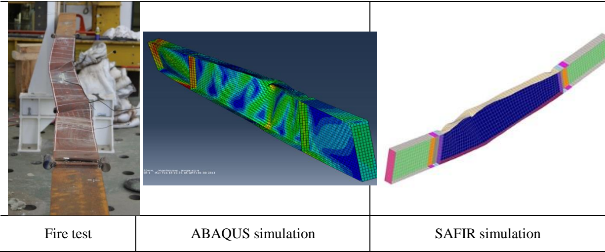
Figure 4: Failure mode shape of the fourth test for LTB – 650 °C
