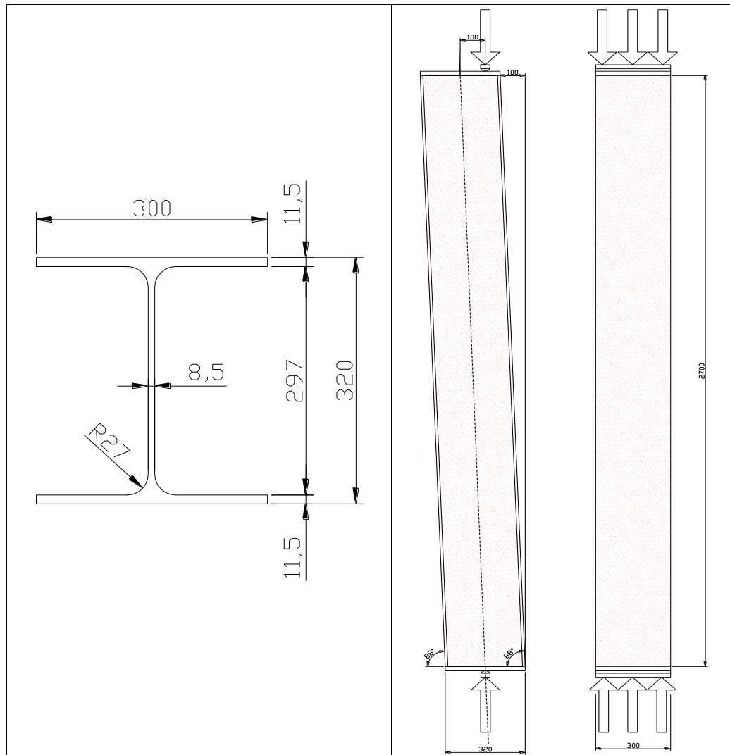
Figure 127: Cross-section design and global design of the test 7
