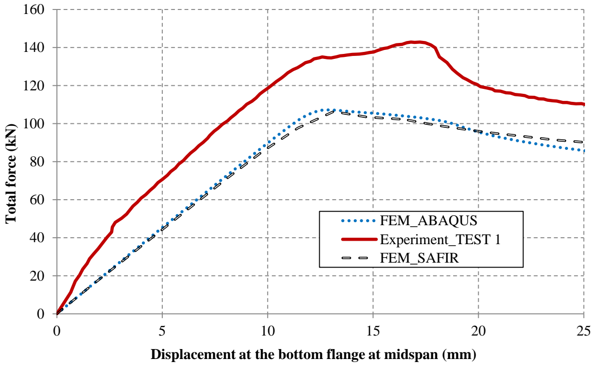
Figure 61: Numerical simulations against experimental fire test
