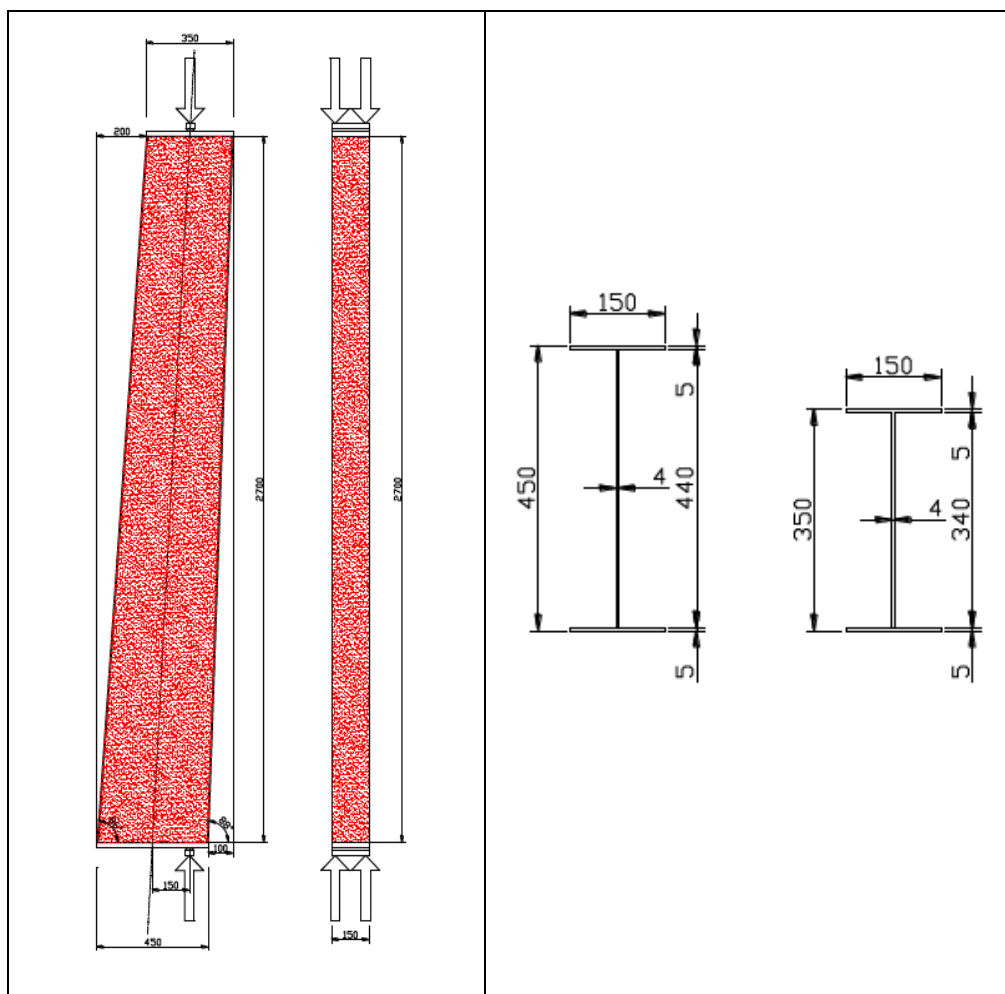
Figure 25: 5th example for benchmark study
