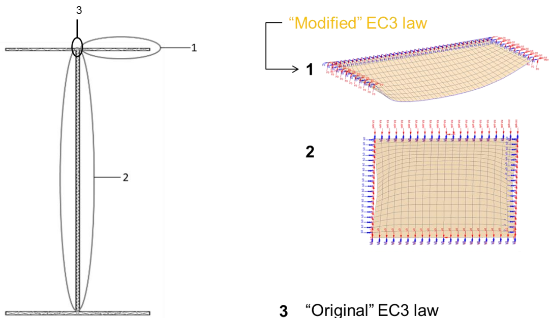
Figure 145: Illustration of buckling with "modified" EC3 law
