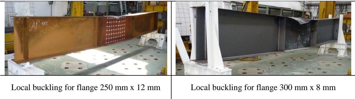
Figure 3: “Intensity” of the local buckling of upper flange according to its width-to-thickness ratio
