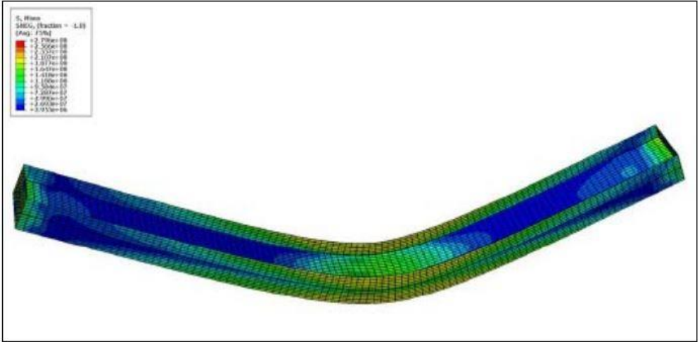
Figure 108: Numerical failure mode obtained with ABAQUS
