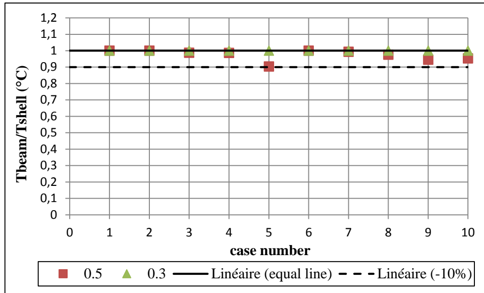
Figure 150: Comparisons between shell and new beam element models for pure bending
