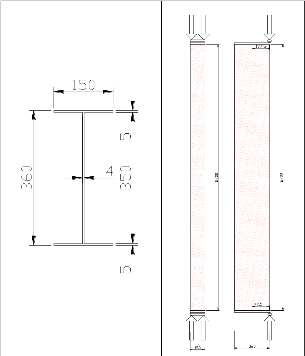
Figure 126: Cross-section design and global design of the tests 6
