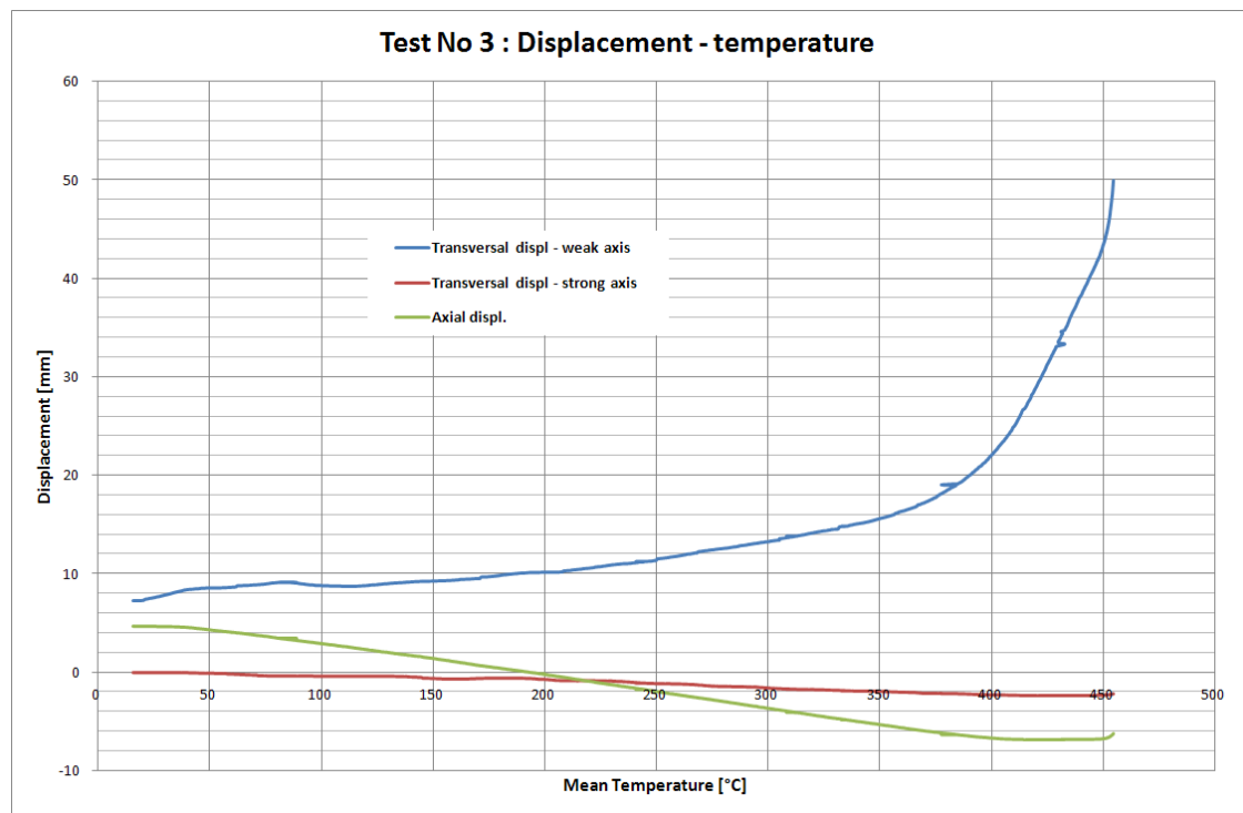
Figure 101: Displacements (mm) in function of the mean temperature (°C)
