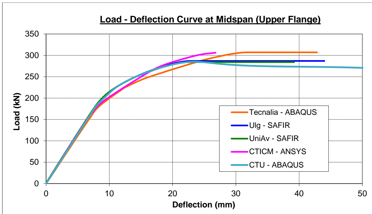
Figure 16: Load-deflection curve at mid-span (upper flange) for 1 st example
