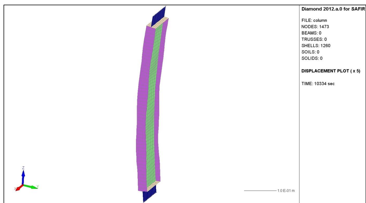
Figure 111: Numerical failure mode obtained with SAFIR
