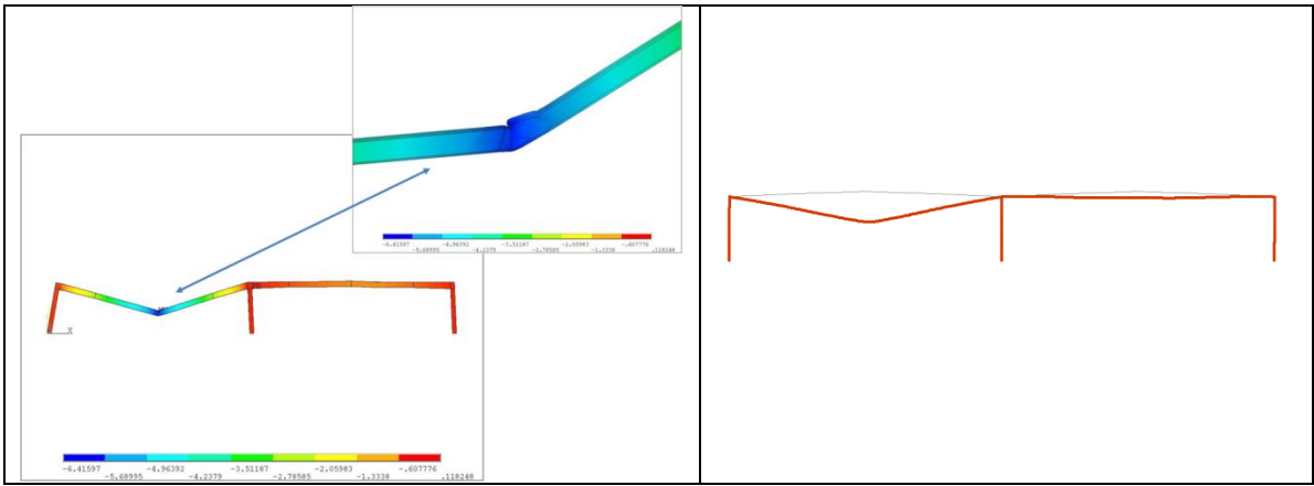
Figure 154: Failure mode for mid-span fire: left) shell model, right) new beam element model
