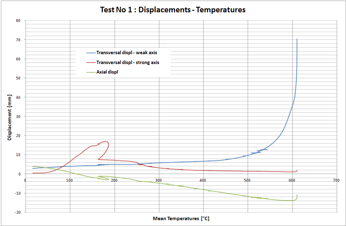
Figure 97: Displacements (mm) in function of the mean temperature (°C)
