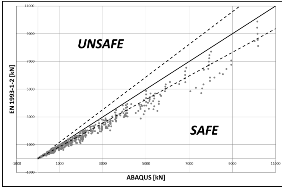
Figure 122: Comparison between EN 1993-1-2 design rules and numerical results for hot-rolled cross-sections
