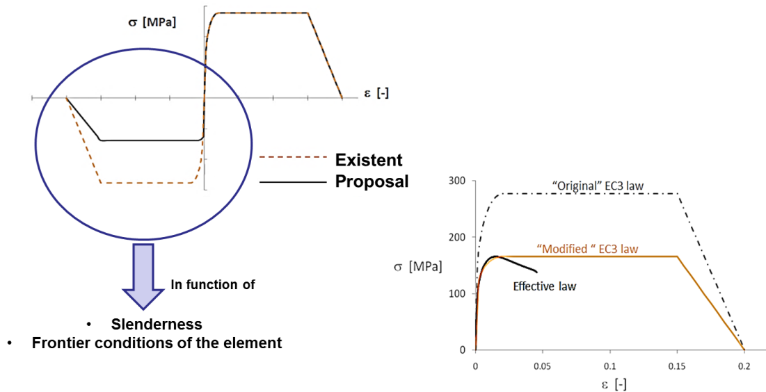
Figure 144: Differences between the material laws
