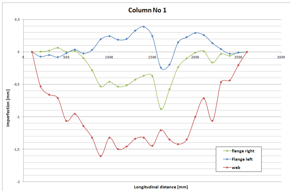
Figure 91: Test 1 – Amplitude of the imperfections along the web and both flanges
