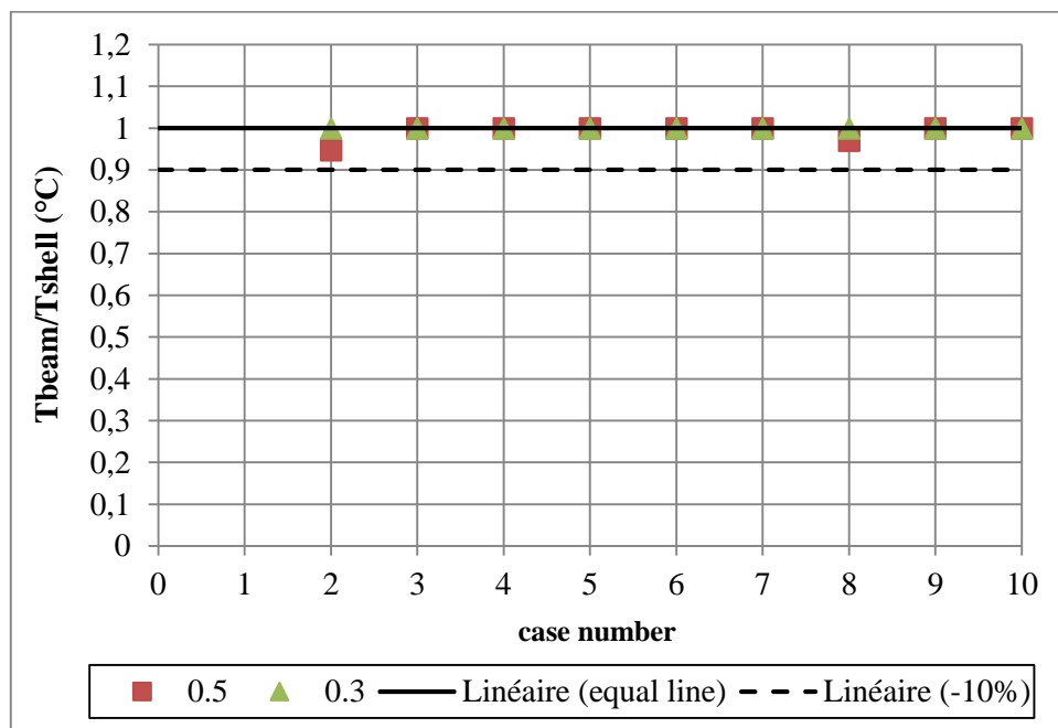
Figure 151: Comparisons between shell and new beam element models for lateral torsional buckling
