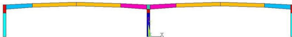
Figure 149: two-span portal frame for the parametric study
