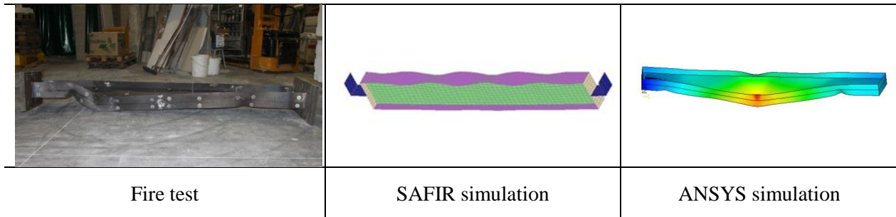
Figure 8: Failure mode shape of the sixth tested beam-column
