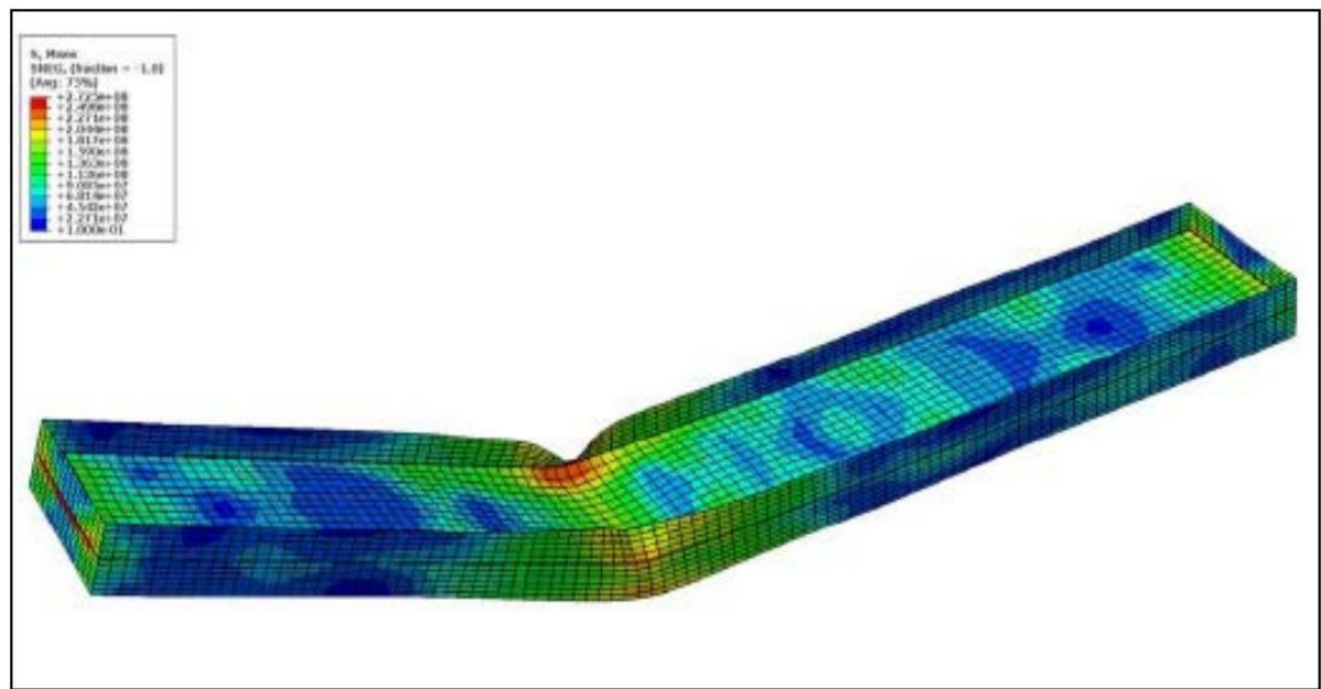
Figure 112: Numerical failure mode obtained with ABAQUS
