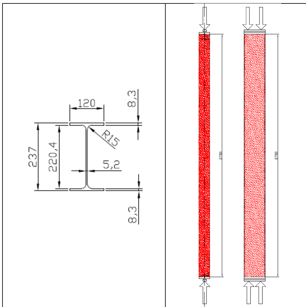
Figure 88: Cross-section design and global design of the test 1
