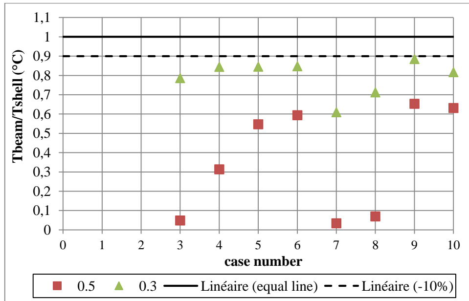
Figure 153: Comparisons between shell and new beam element models for columns subjected to combined axial load and bending moment
