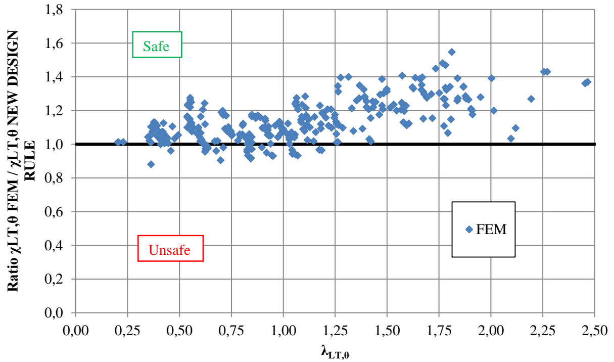
Figure 87: Tapered beams; comparison between numerical results and new design rule
