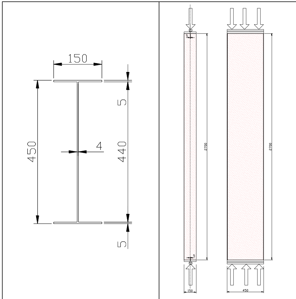
Figure 89: Cross-section design and global design of the tests 2 & 3
