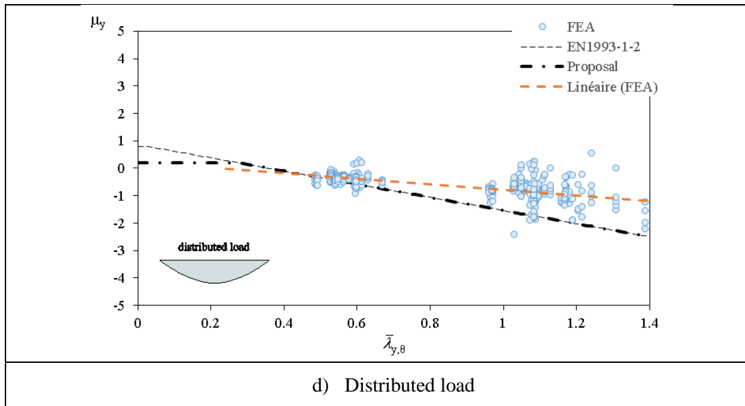
Figure 134: Calibration of factor \mu_y for the in-plane behaviour of beam-columns considering different loading cases
