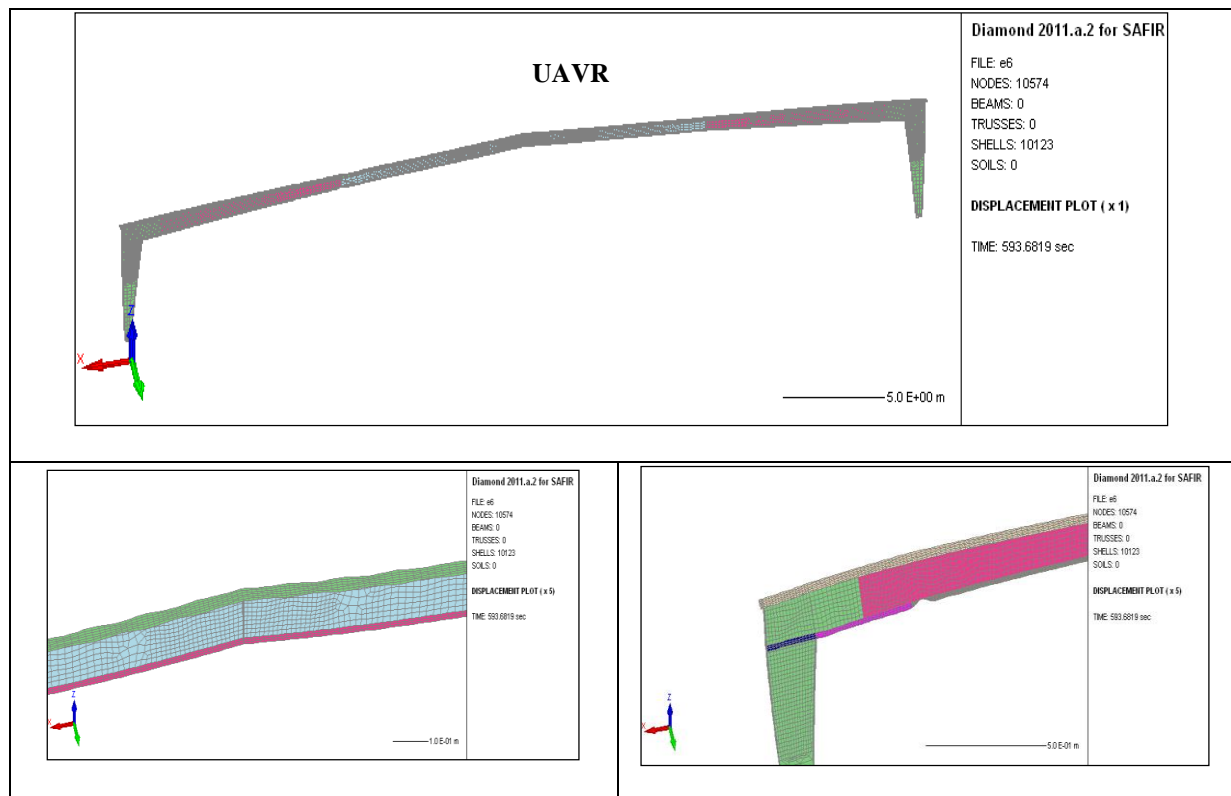
Figure 32: Failure mode of the frame obtained with the different computer codes
