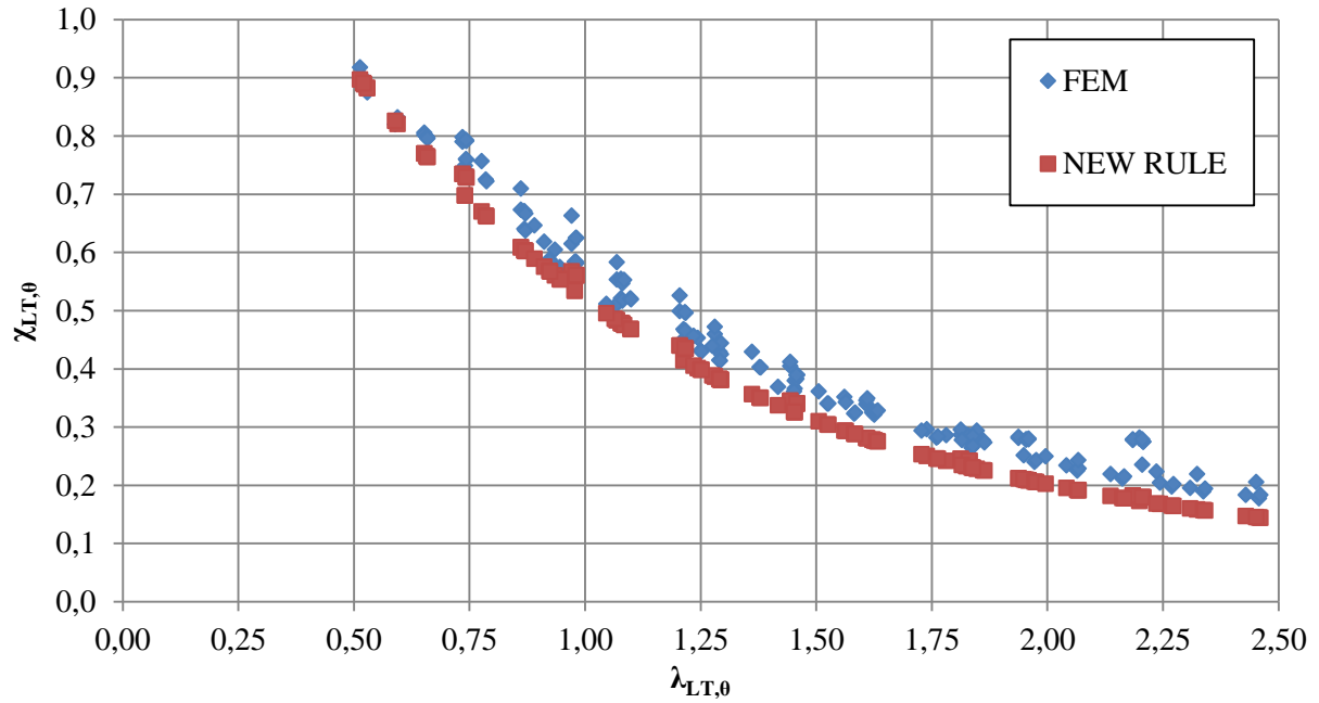
Figure 80: Comparison between the results of the parametric study and the new proposed design procedure for triangular bending moment and curve L1
