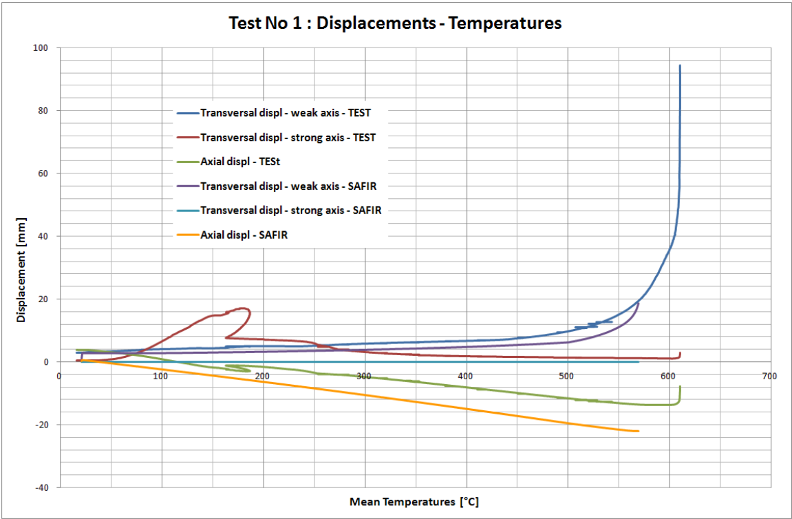
Figure 105: Displacements (mm) in function of temperature (°C) – SAFIR comparison
