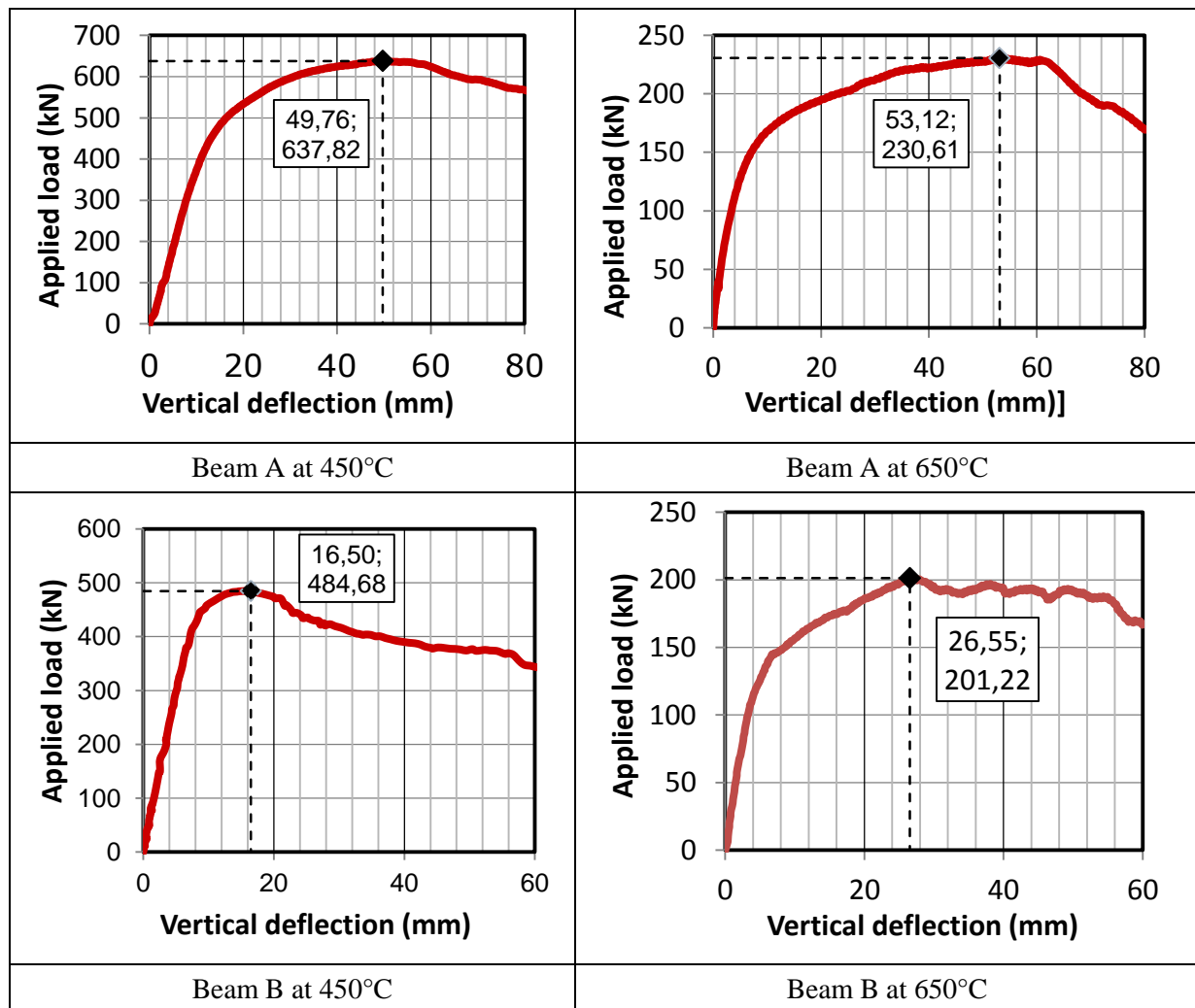
Figure 35: Recorded load-deflection curves of four tested beams
