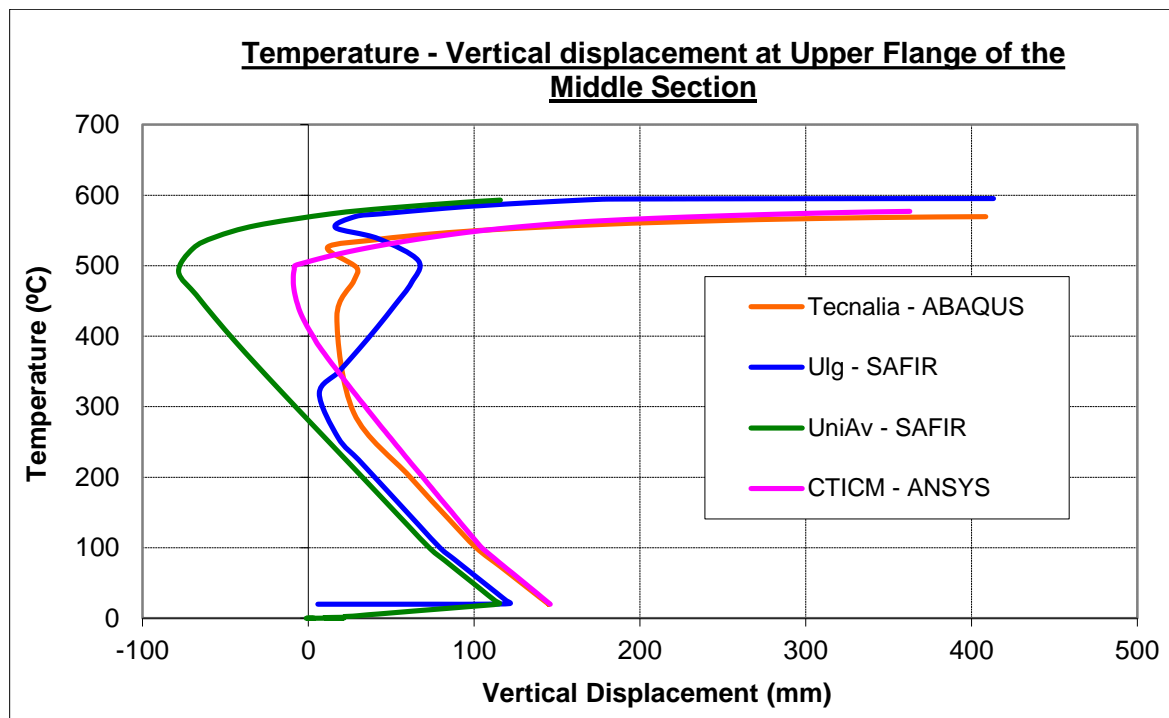
Figure 31: Temperature – vertical displacement at upper flange of the middle section of the frame
