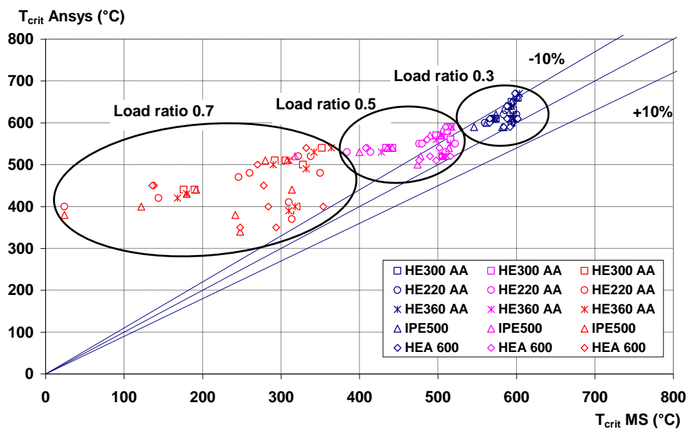
Figure 12: Comparison of critical temperatures between simple calculation method ( T_{crit} MS) and advanced numerical model ( T_{crit} ANSYS)
