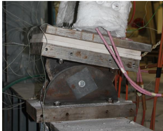
Figure 94: Pinned support with thermal disconnection
