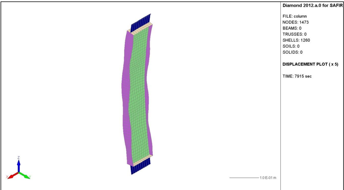
Figure 115: Numerical failure mode obtained with SAFIR
