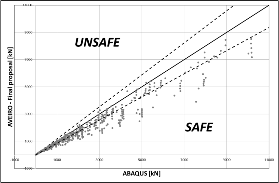
Figure 124: Comparison between new design rules and numerical results for hot-rolled cross-sections
