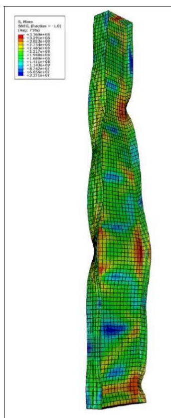
Figure 120: Numerical failure mode obtained with ABAQUS
