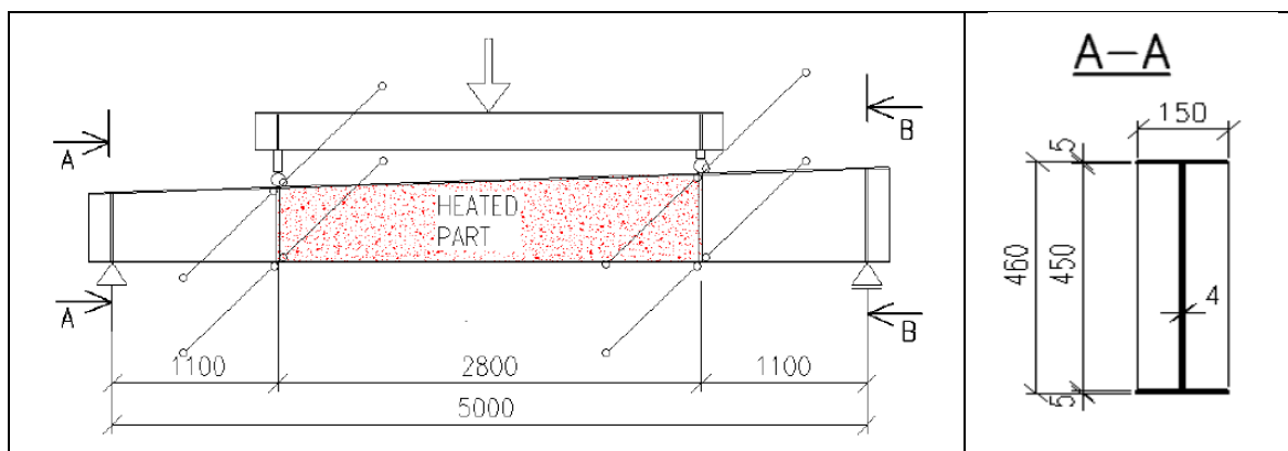
Figure 19: 3 rd example for benchmark study
