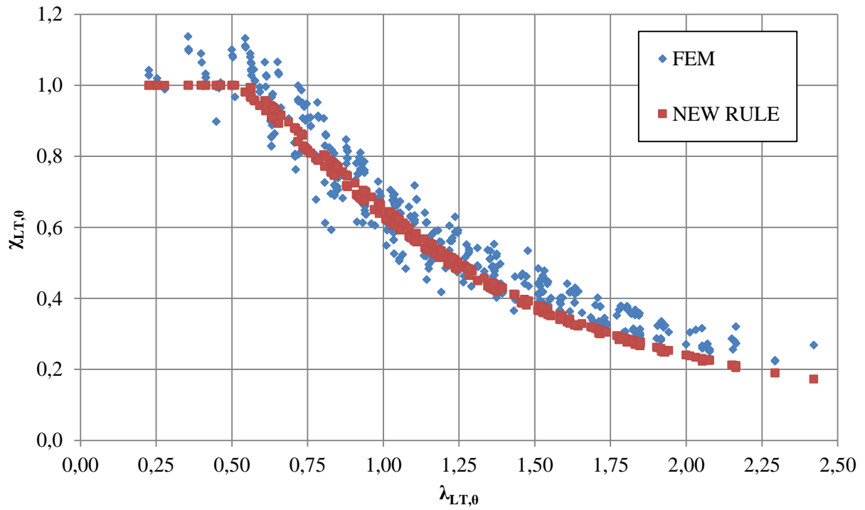
Figure 85: Comparison between the results of the parametric study and the new proposed design procedure for bi-triangular bending moment and curve L3
