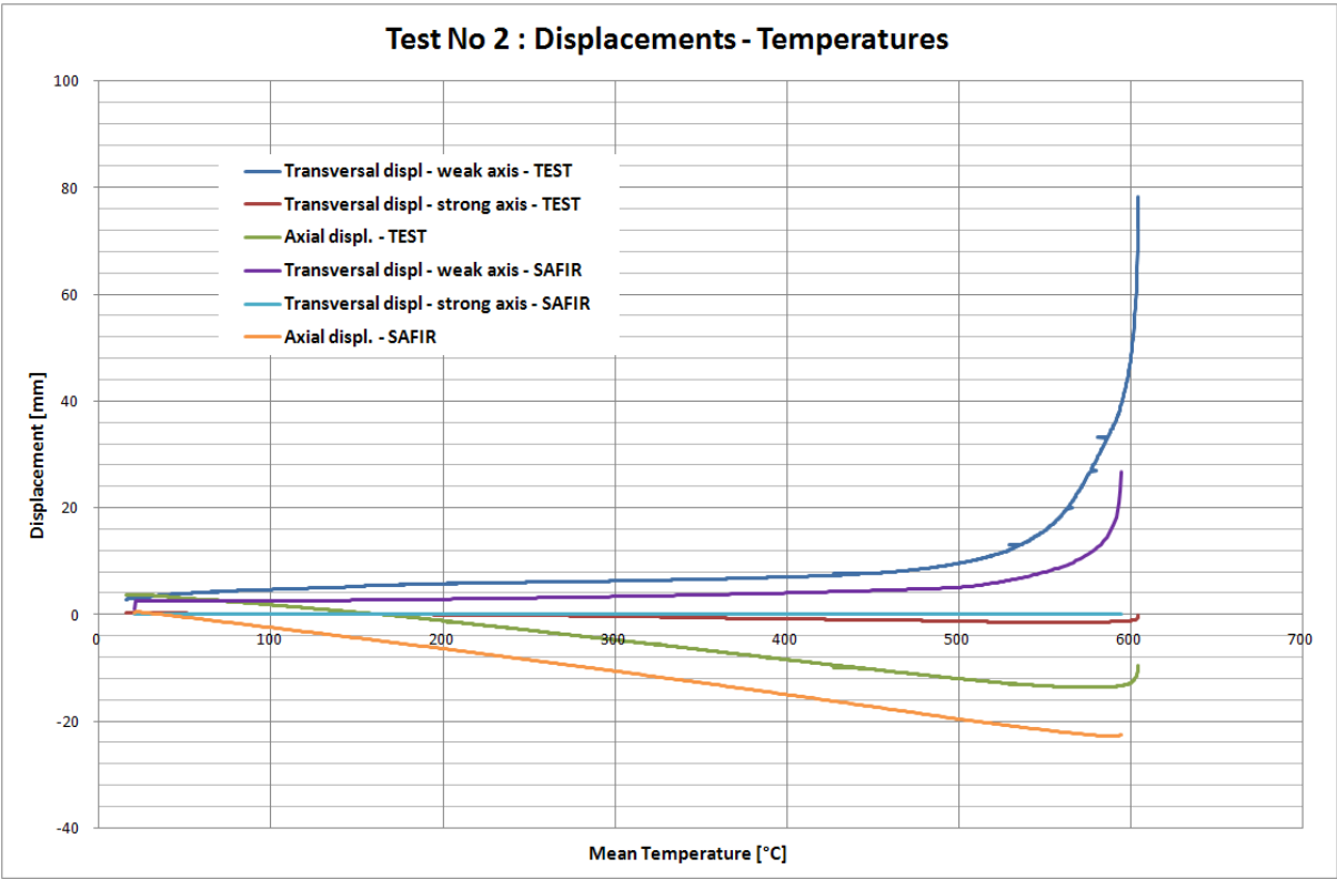
Figure 109: Displacements (mm) in function of temperature (°C) – SAFIR comparison
