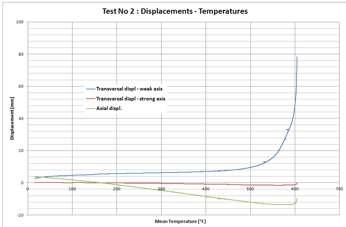
Figure 99: Displacements (mm) in function of the mean temperature (°C)
