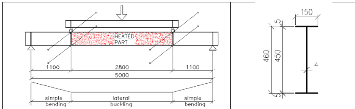
Figure 18: 2 nd example for benchmark study
