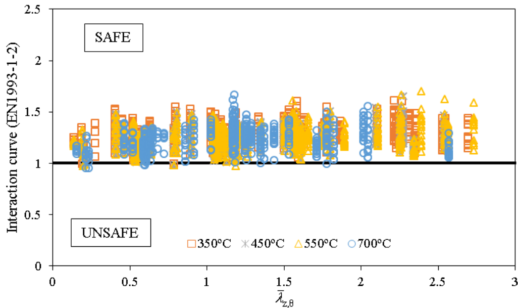
Figure 132: Comparison of interaction curve and the numerical cases studied for the out-of-plane behaviour in terms of non-dimensional slenderness
