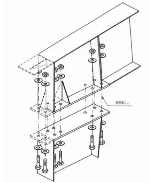
Figure 14 : Typical knee connection
