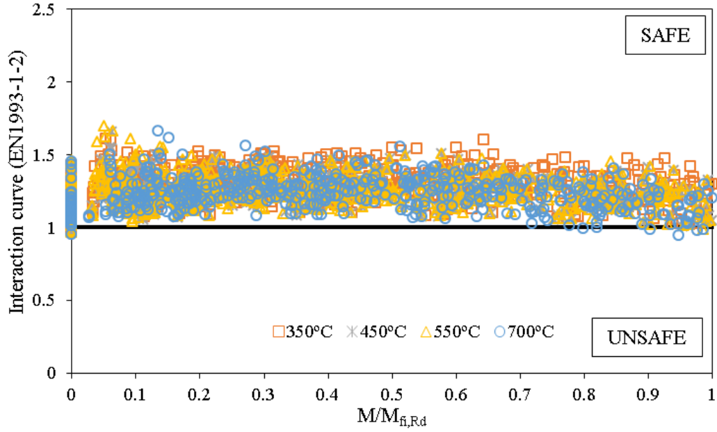
Figure 133: Comparison of interaction curve and the numerical cases studied for the out-of-plane behaviour in terms of the applied bending moment
