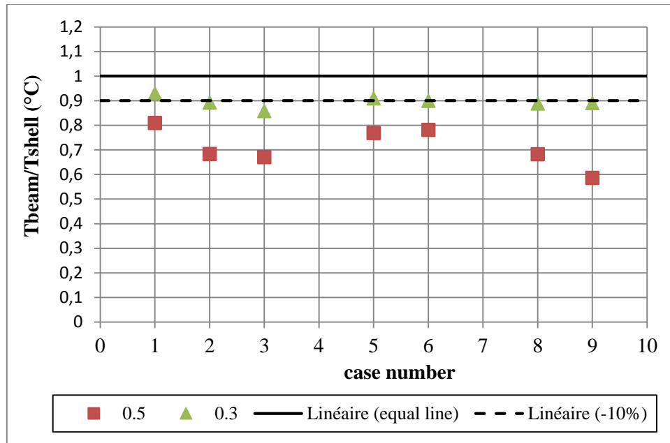
Figure 152: Comparisons between shell and new beam element models for axially loaded columns
