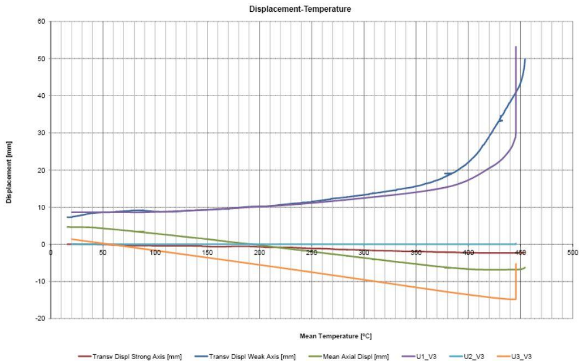
Figure 114: Displacements (mm) in function of temperature (°C) – ABAQUS comparison
