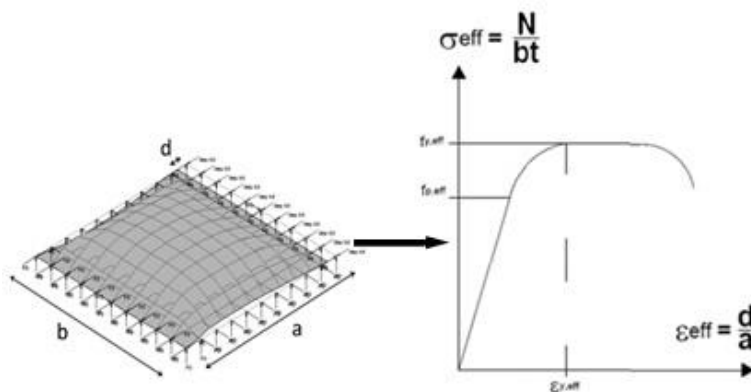
Figure 143: Illustration of the applied method to get the new material law
