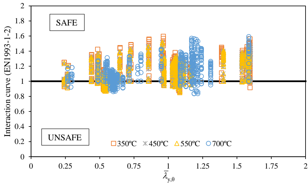
Figure 130: Comparison of the numerical analysis results with the EN 1993-1-2 interaction curve for various temperatures a function of the beam-column slenderness
