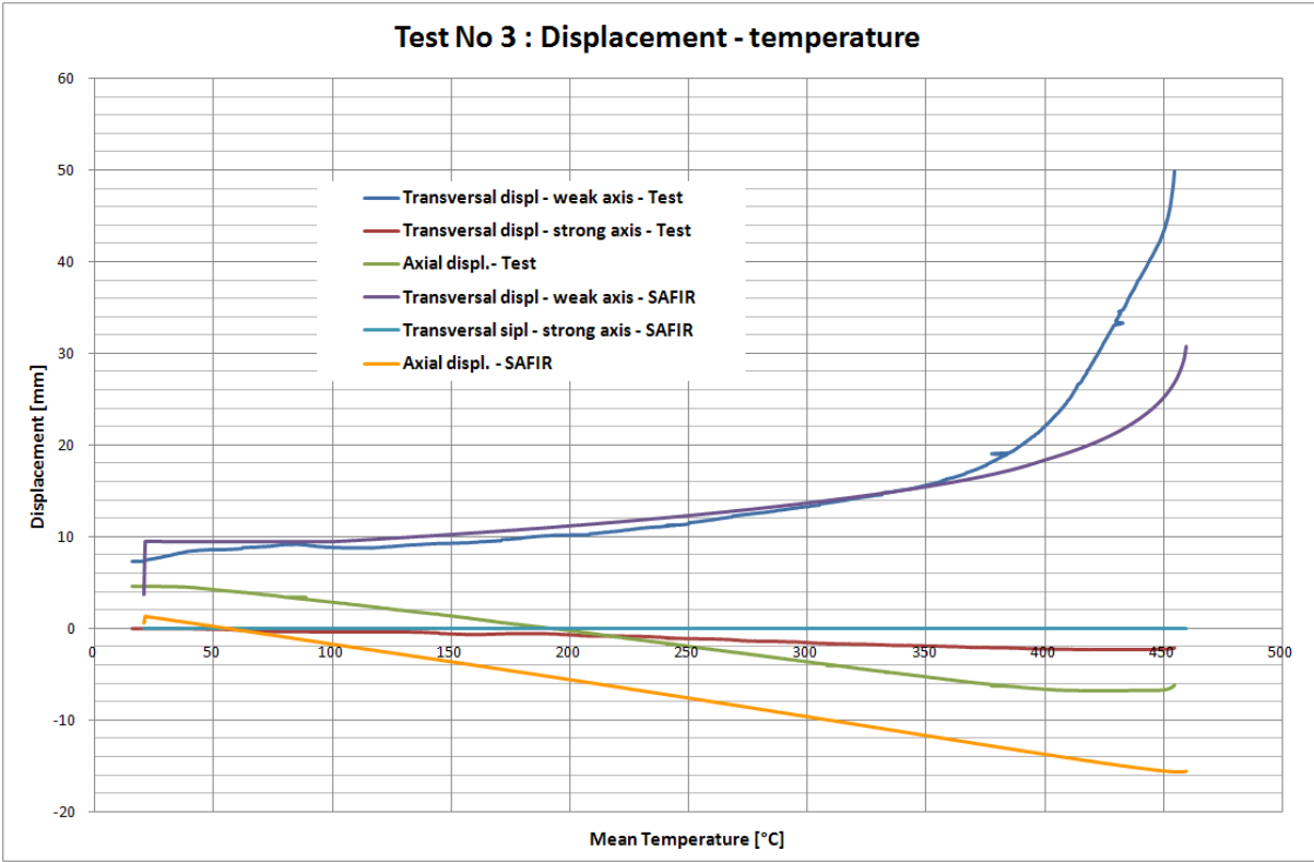
Figure 113: Displacements (mm) in function of temperature (°C) – SAFIR comparison
