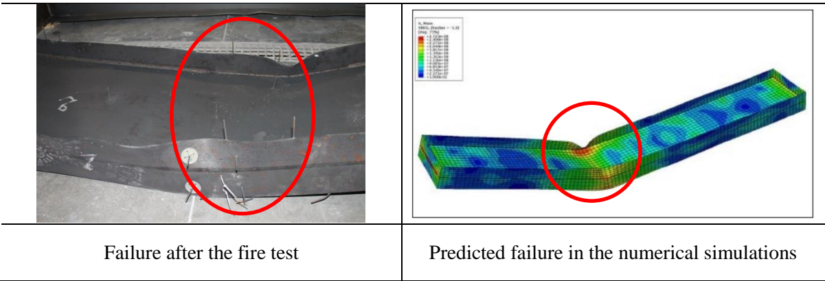
Figure 7: Failure of test 2 for both numerical simulations and experimentation
