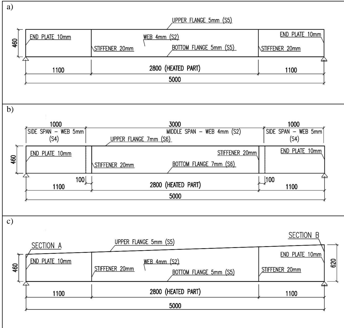
Figure 53: Tested beams: a) tests 1 & 2, b) test 3, c) test 4
