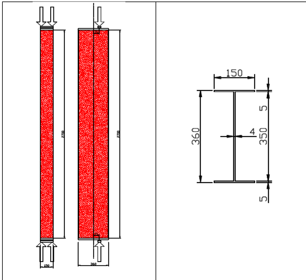
Figure 24: 4 th example for benchmark study
