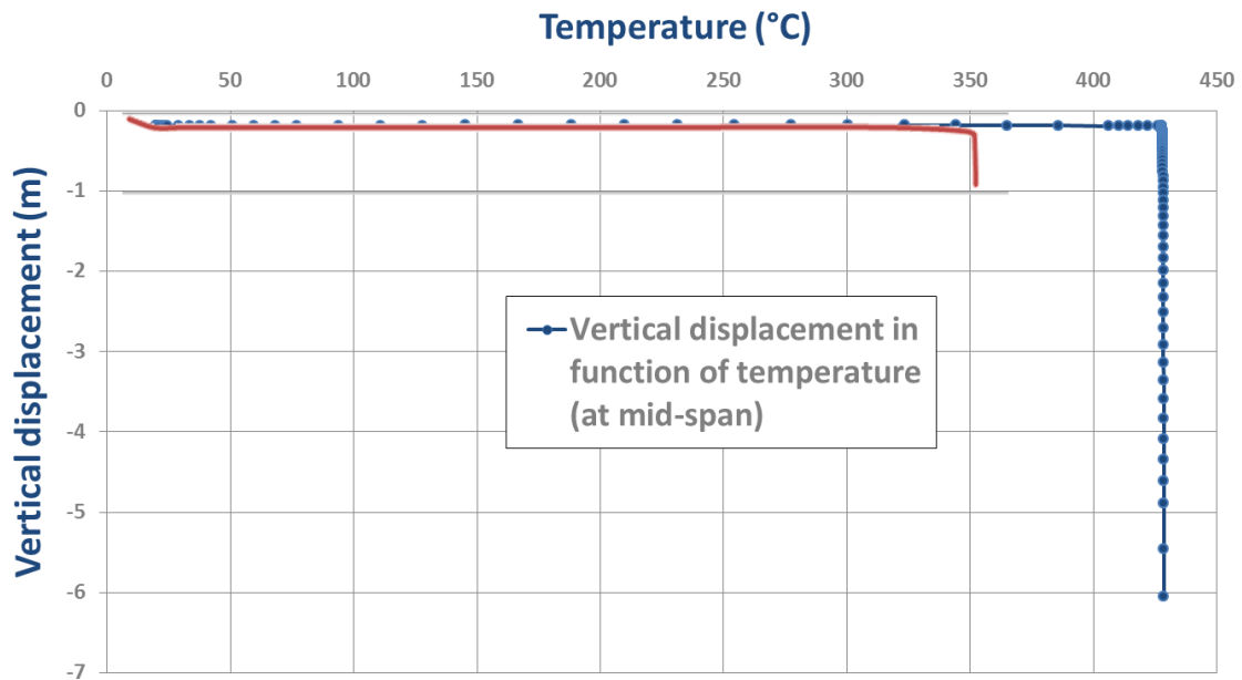
Figure 156: Vertical displacement (m) in function of temperature (°C) at mid span (red is beam model, blue is shell model)
