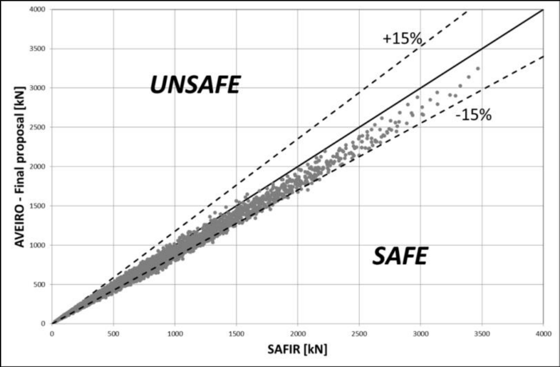
Figure 123: Comparison between new design rules and numerical results for welded cross-sections
