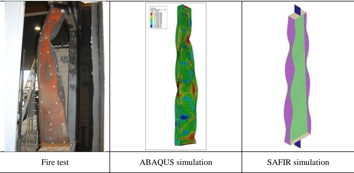
Figure 5: Failure mode shape of the fourth test for axially loaded column
