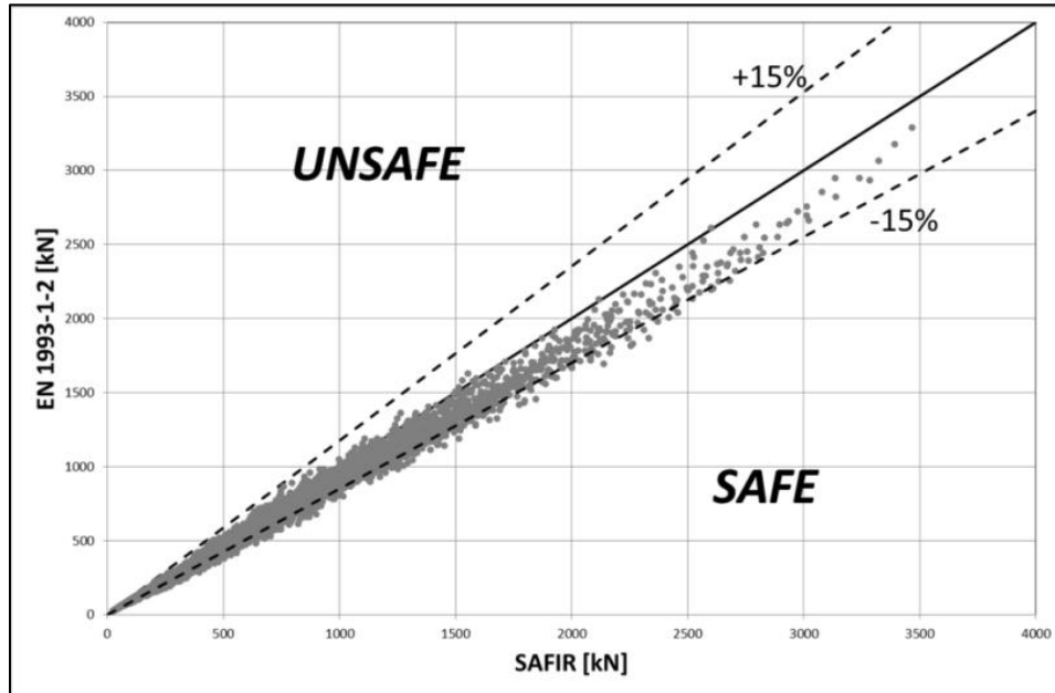
Figure 121: Comparison between EN 1993-1-2 design rules and numerical results for welded cross-sections
