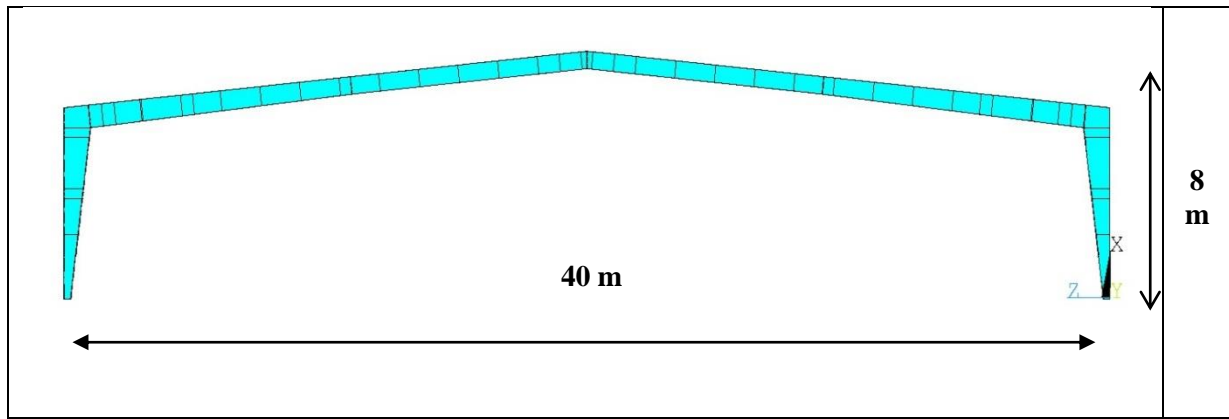
Figure 30: 6 th example for benchmark study
