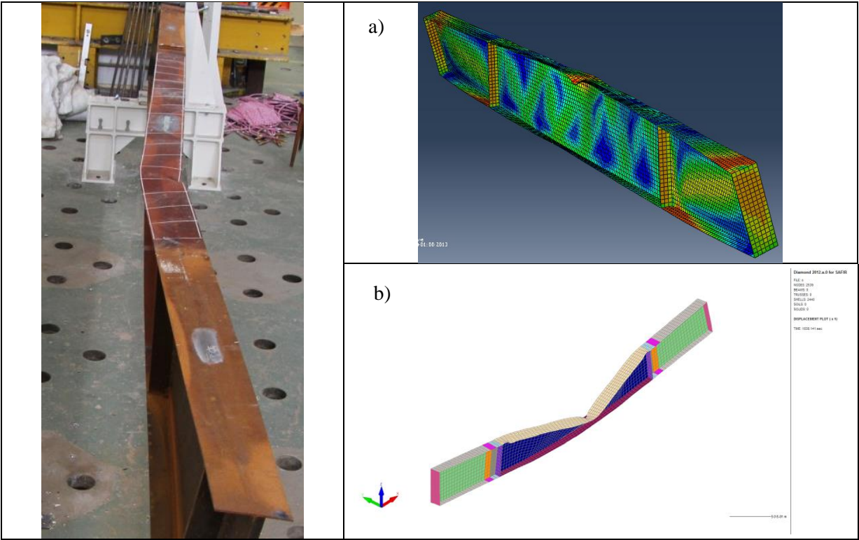
Figure 62: Failure mode shape for fire test and numerical simulation with: a) ABAQUS, b) SAFIR
