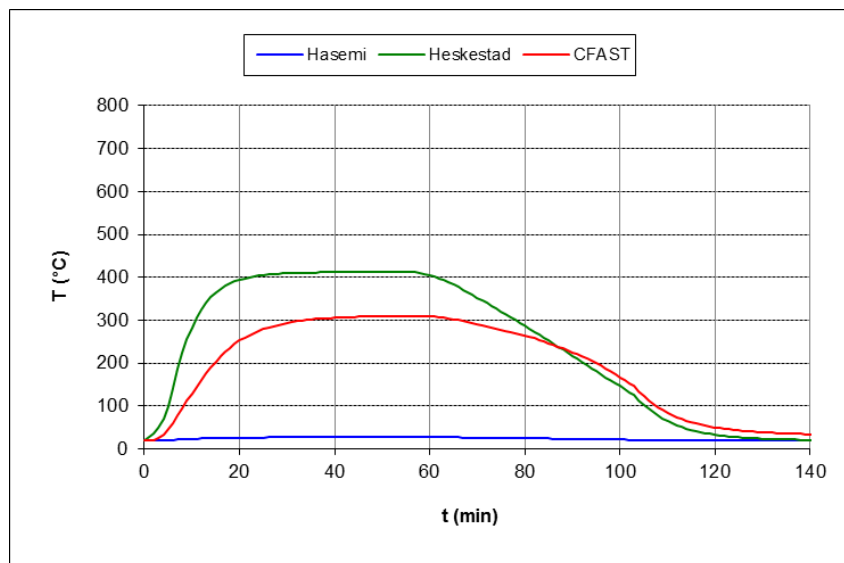
Figure 146: Evolution of temperature in function of time in the selected real fire scenario
