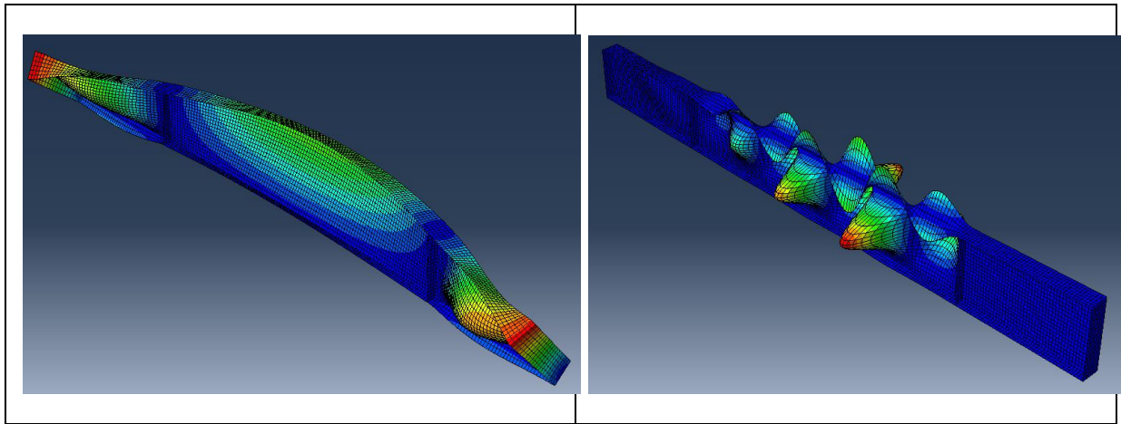
Figure 70: Mode shape from linear buckling analysis: left) lateral torsional buckling failure mode, right) local buckling failure mode
