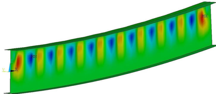
Figure 49: Deformed shape of a class 4 cross-section with class 2 flanges
