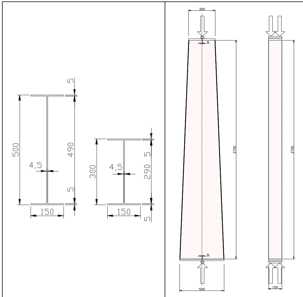
Figure 90: Cross-section design and global design of the test 4
