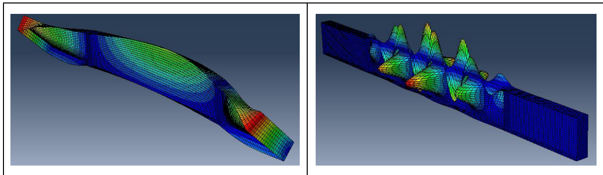
Figure 60: Mode shape from linear buckling analysis: left) lateral torsional buckling failure mode, right) local buckling failure mode
