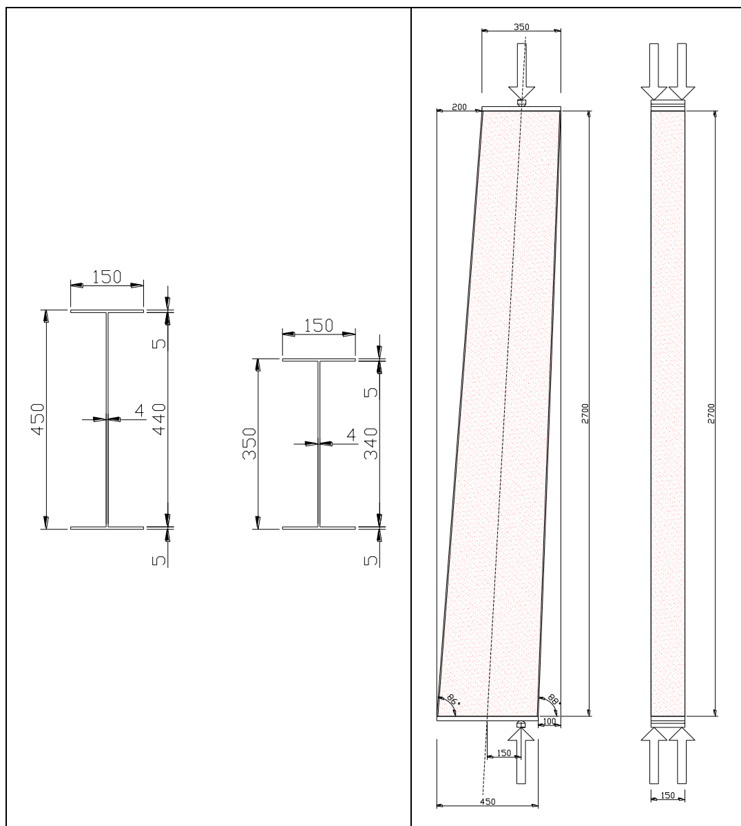
Figure 128: section design and global design of the test 8
