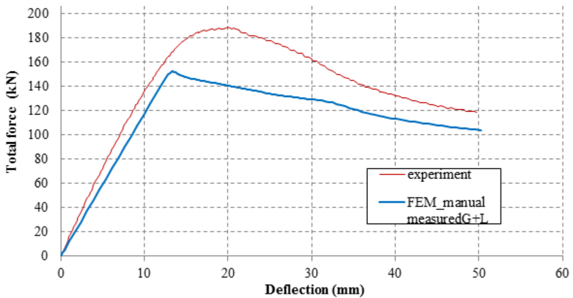
Figure 68: Numerical simulations against experimental fire test
