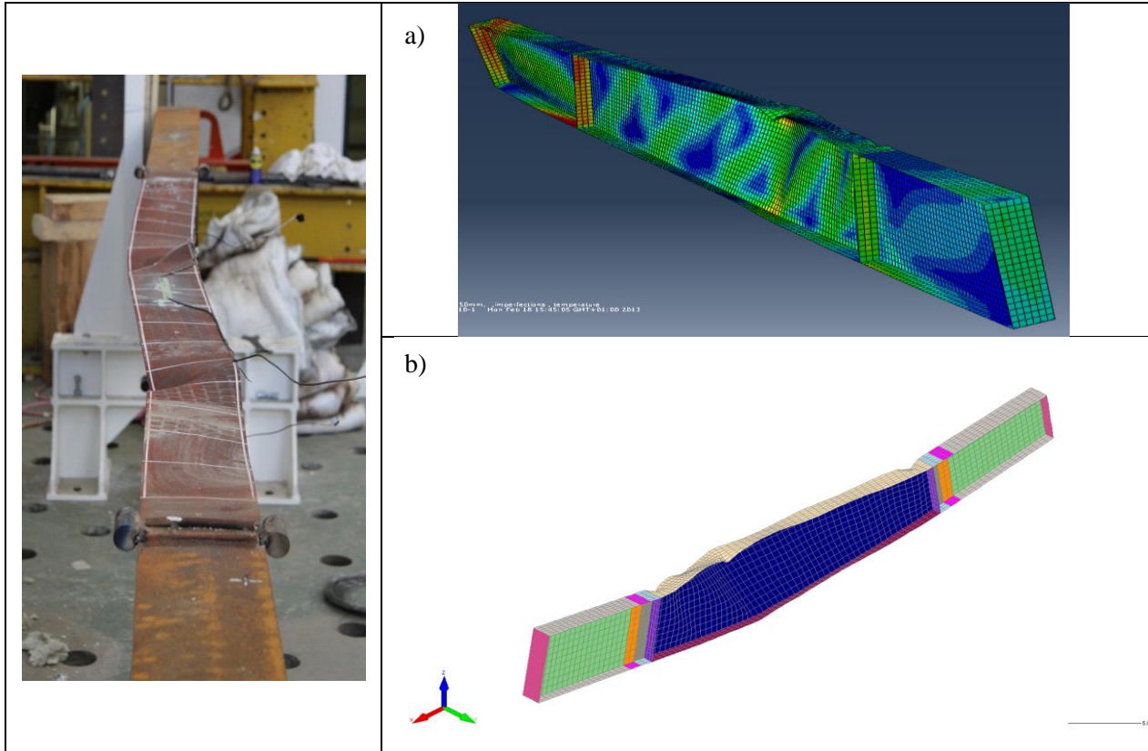
Figure 72: Failure mode shape for fire test and numerical simulation with: a) ABAQUS, b) SAFIR
