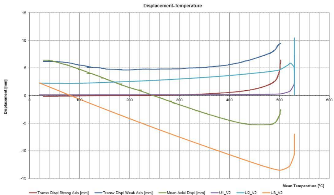
Figure 118: Displacements (mm) in function of temperature (°C) – ABAQUS comparison
