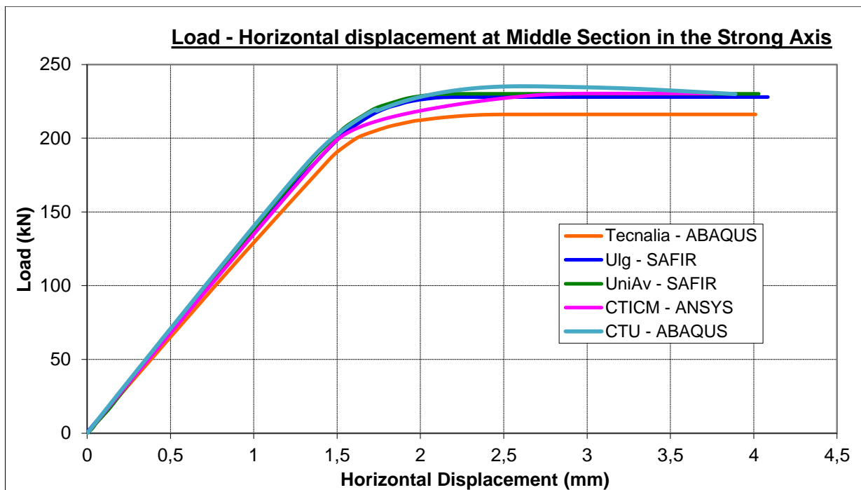
Figure 27: Load – horizontal displacement at middle section in the strong axis for 5 th example
