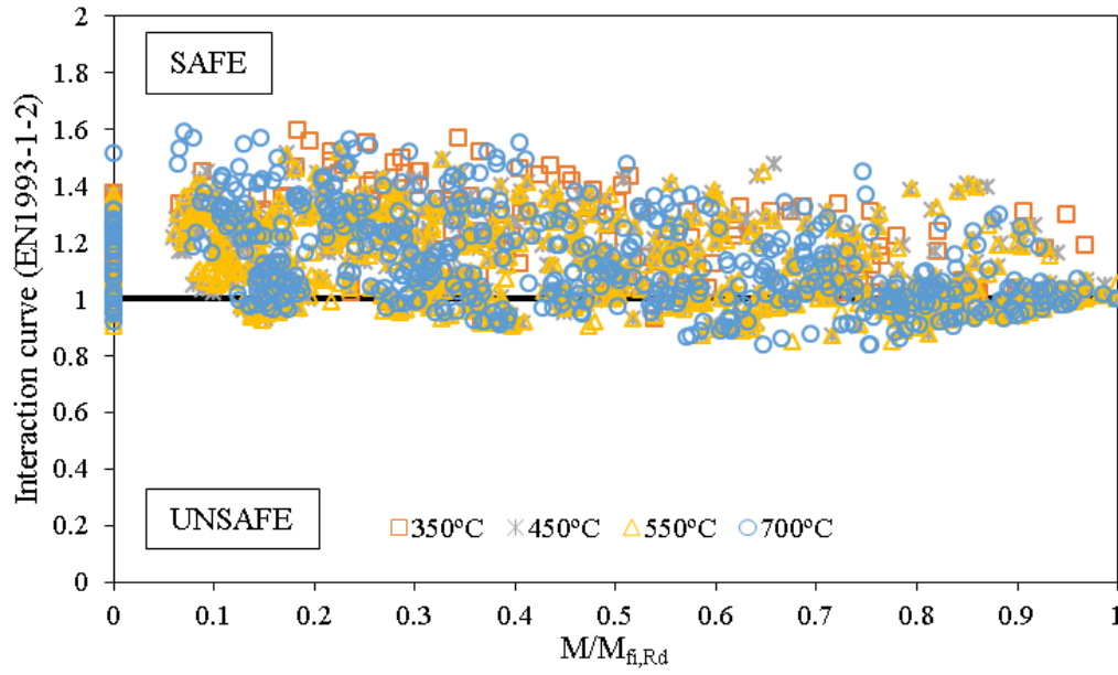
Figure 131: Comparison of the numerical analysis with the EN 1993-1-2 interaction curve for various temperatures as a function of the applied bending moment
