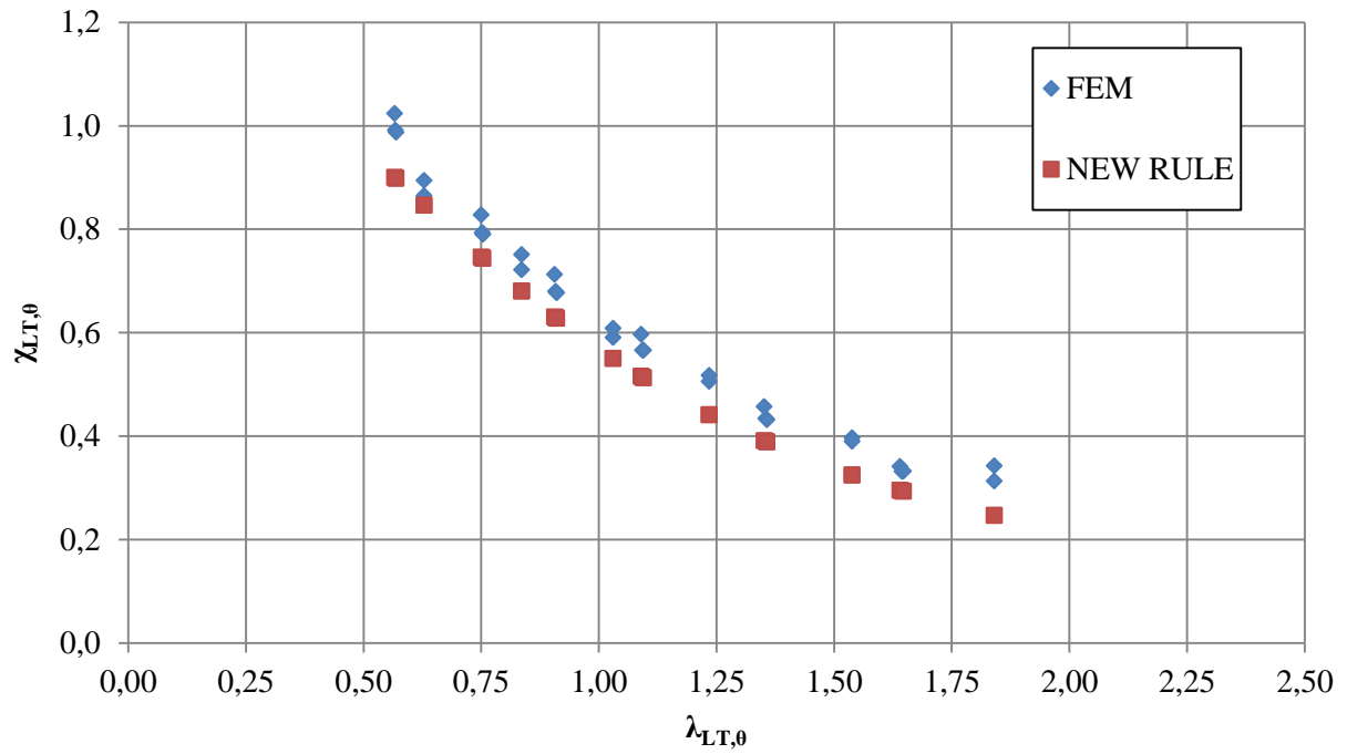
Figure 84: Comparison between the results of the parametric study and the new proposed design procedure for bi-triangular bending moment and curve L2
