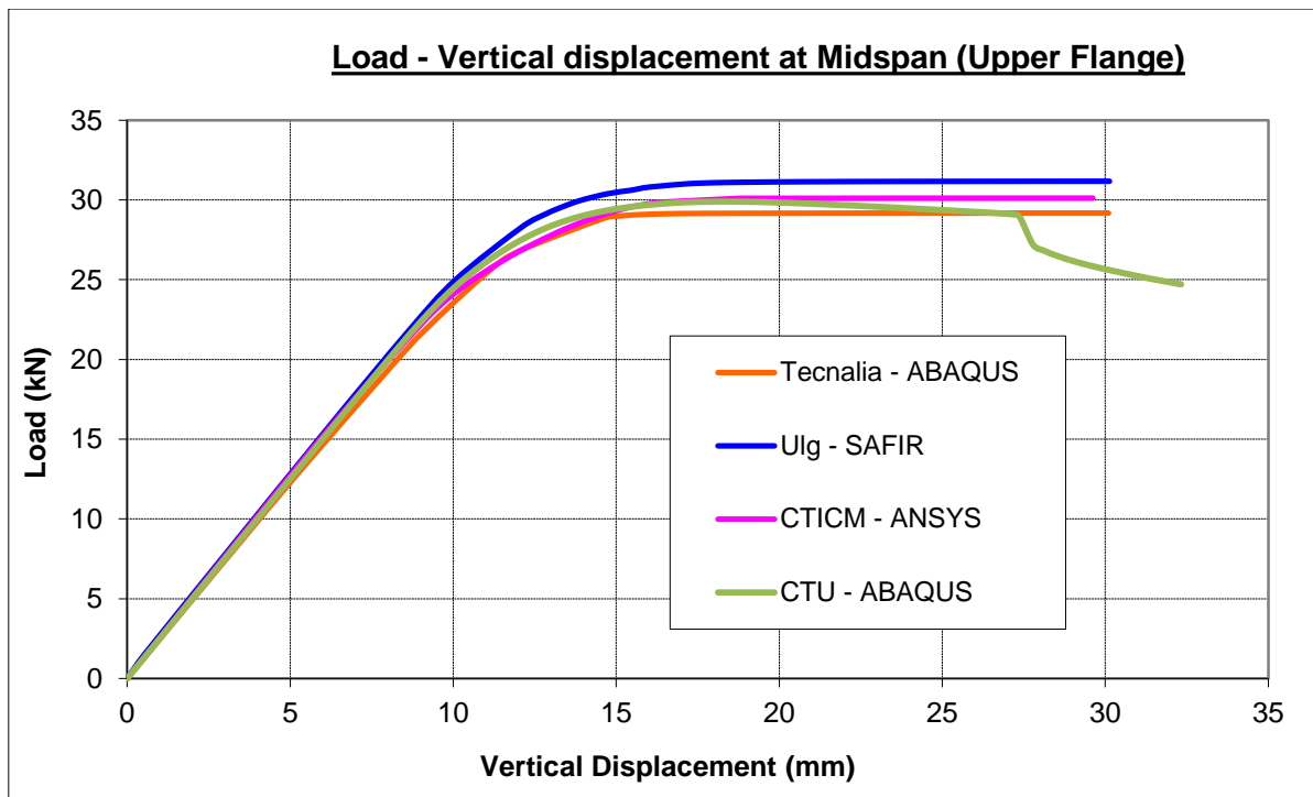
Figure 21: Load-deflection curve at mid-span (upper flange) for 3 rd example
