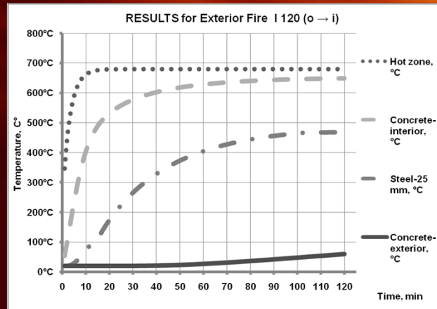
Graph of the calculation of the unstationary heat conduction
